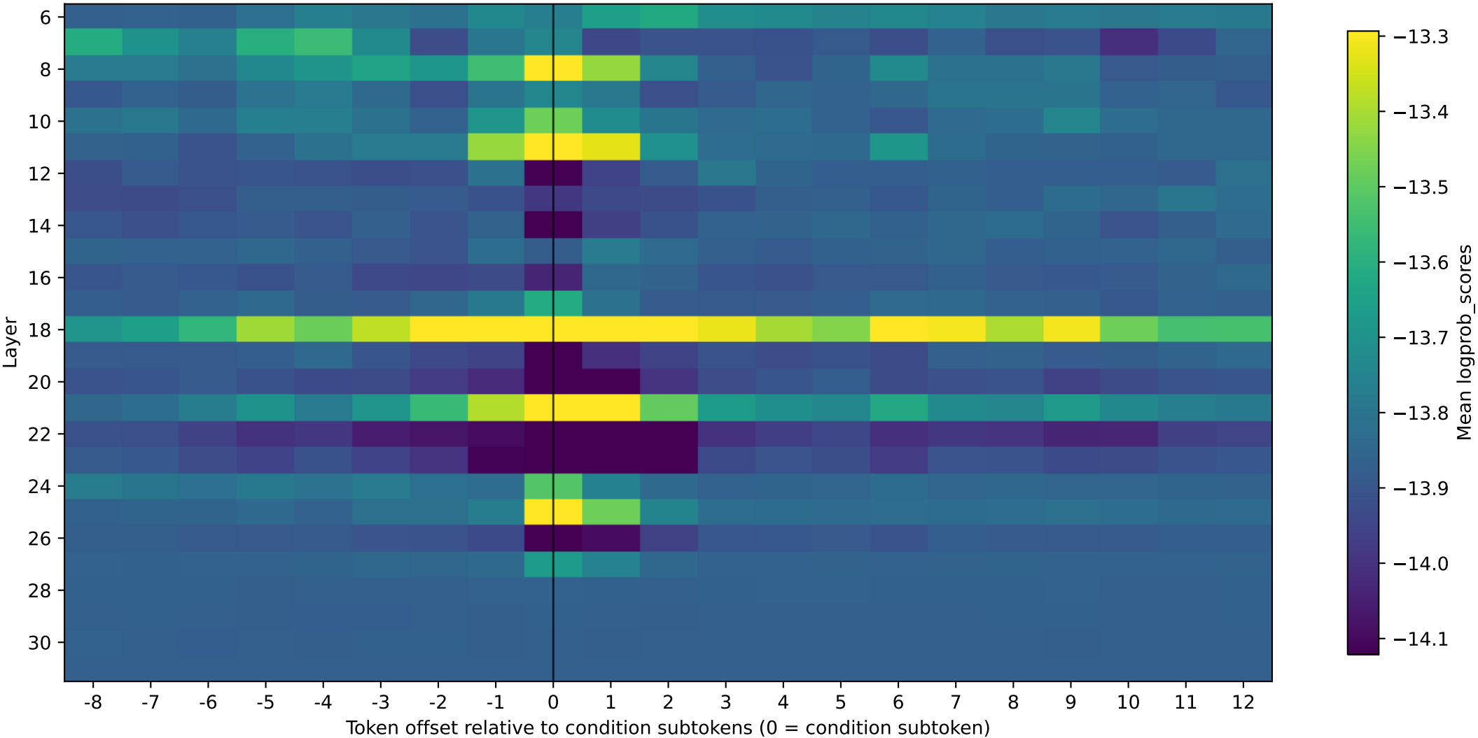
OLMo all 155 units: condition-aligned mean logprob scores
