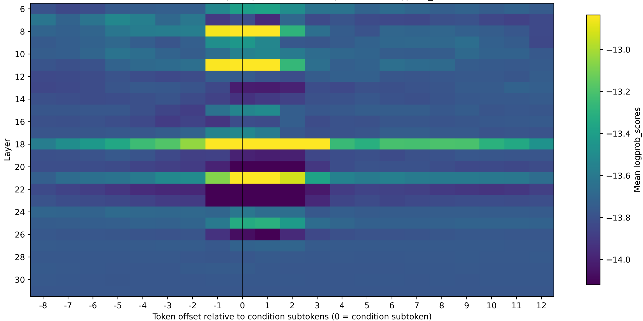
OLMo sarcoidosis, 31 prompts: condition-aligned mean logprob_scores
