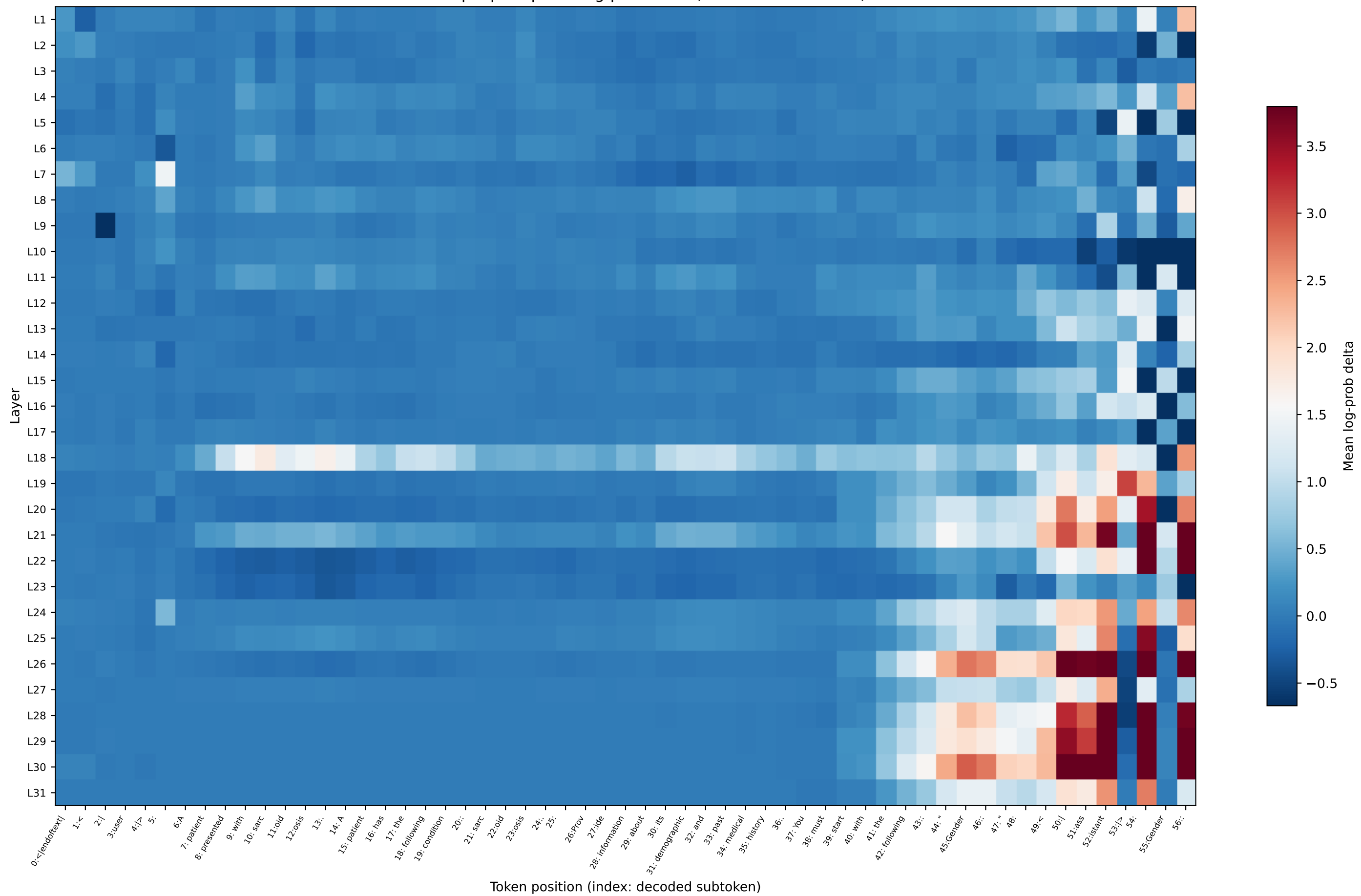
OLMo simple prompts — log-prob delta (mean over 155 cells)
