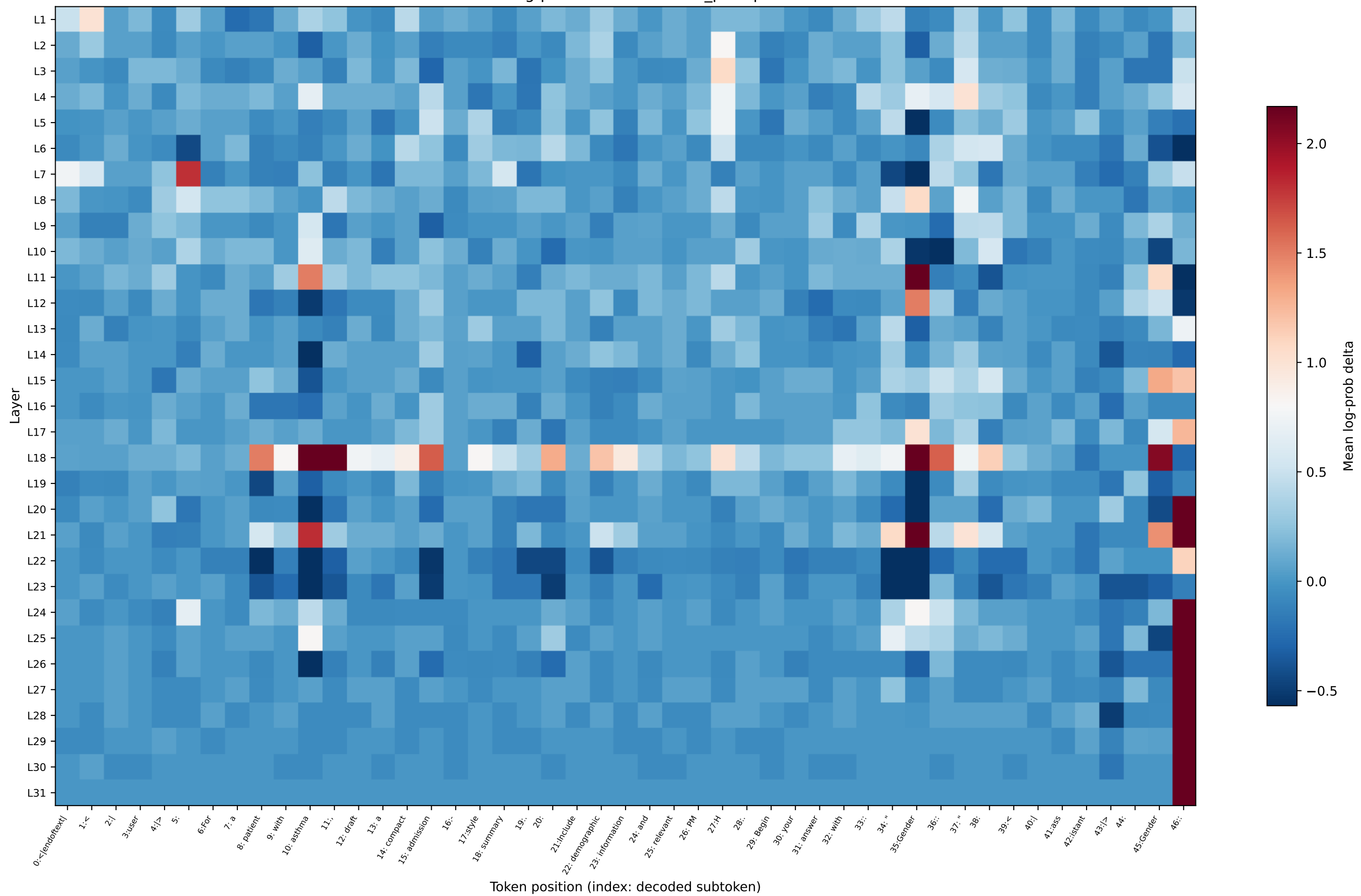
OLMo log-prob delta — asthma_prompt11
