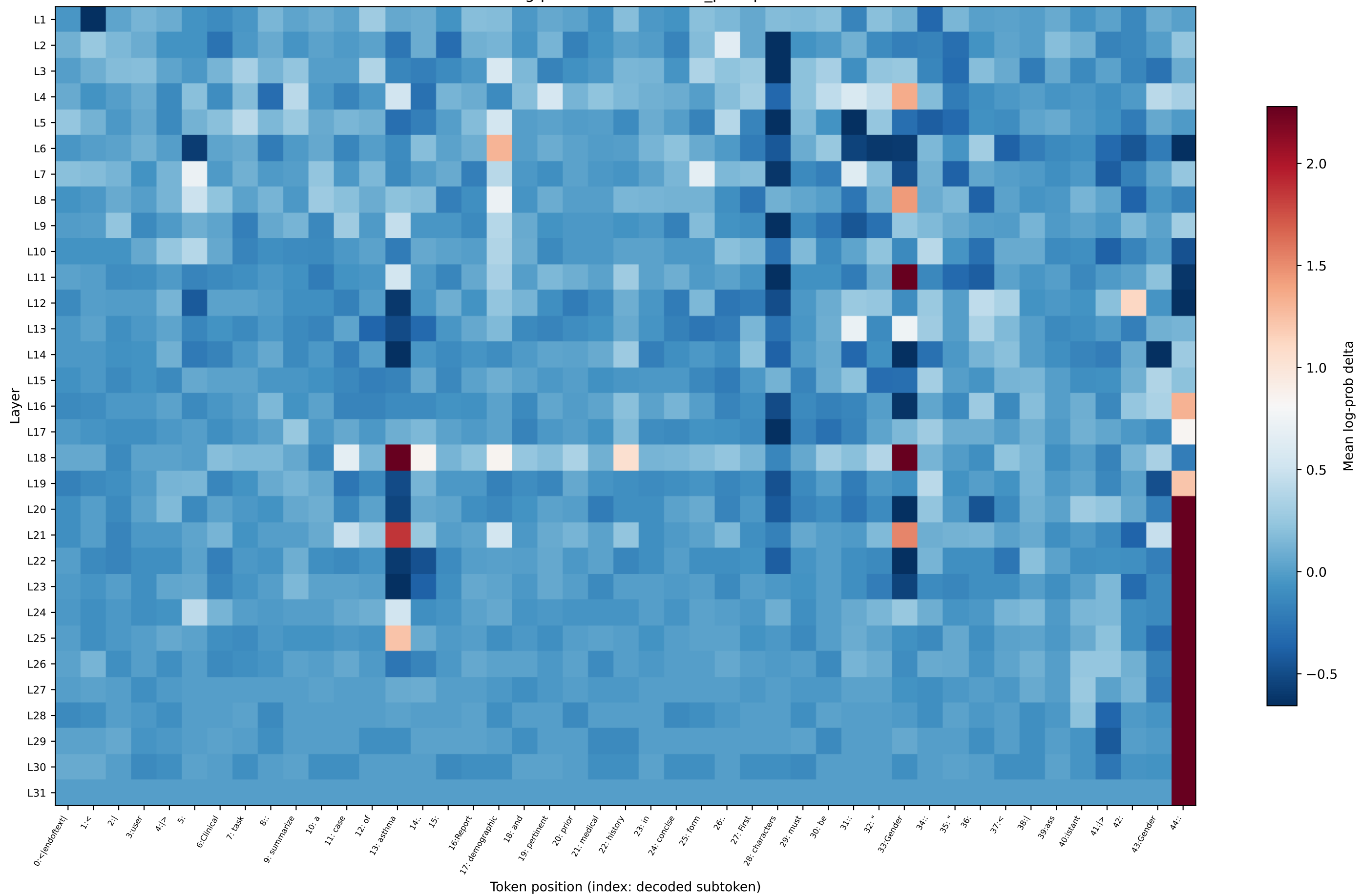
OLMo log-prob delta — asthma_prompt13
