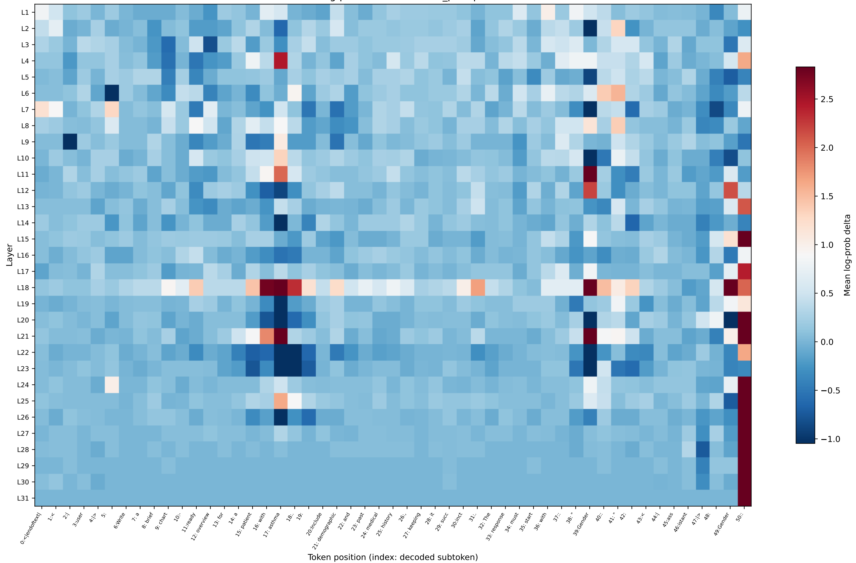
OLMo log-prob delta — asthma_prompt17
