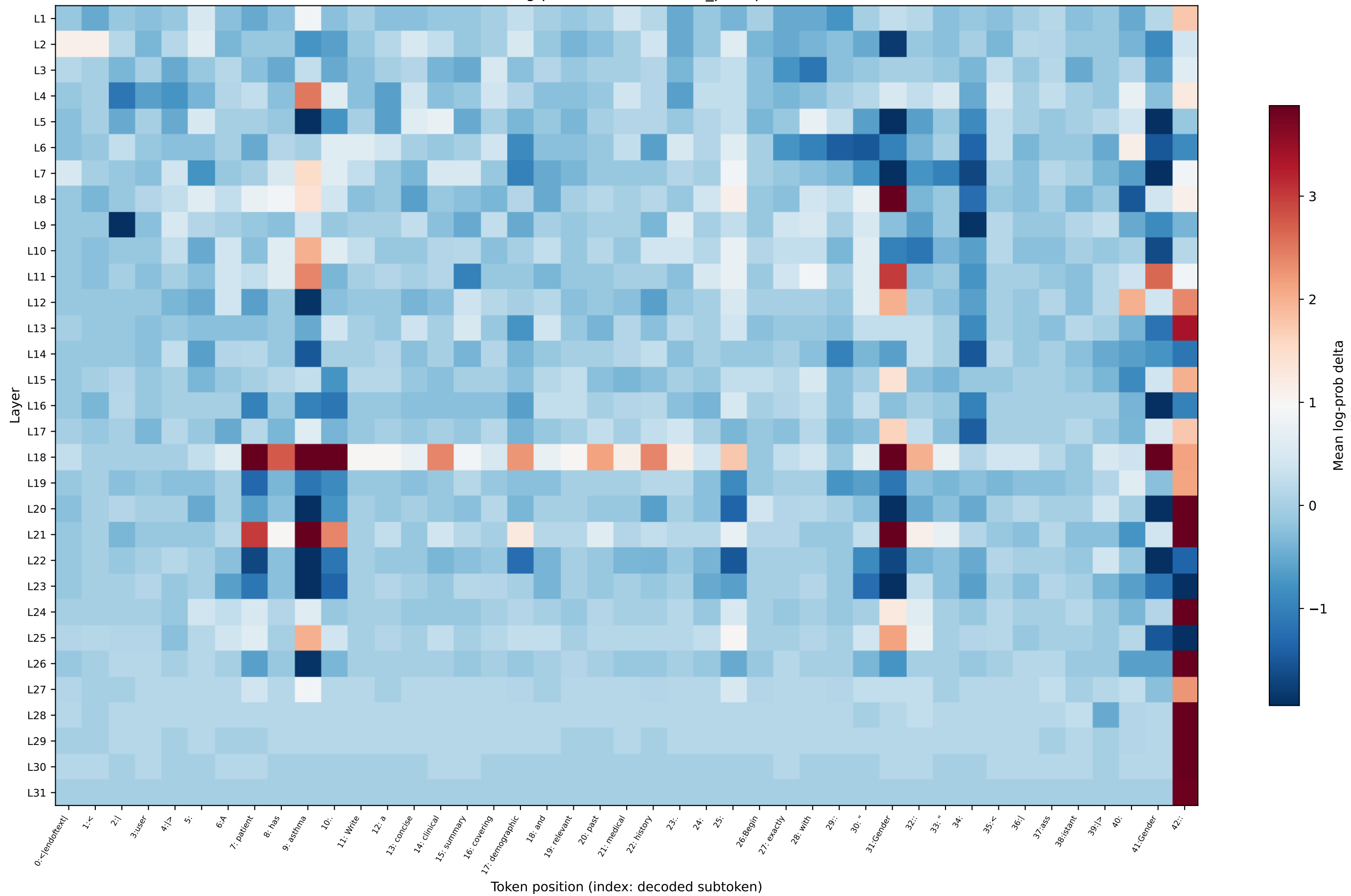
OLMo log-prob delta — asthma_prompt18
