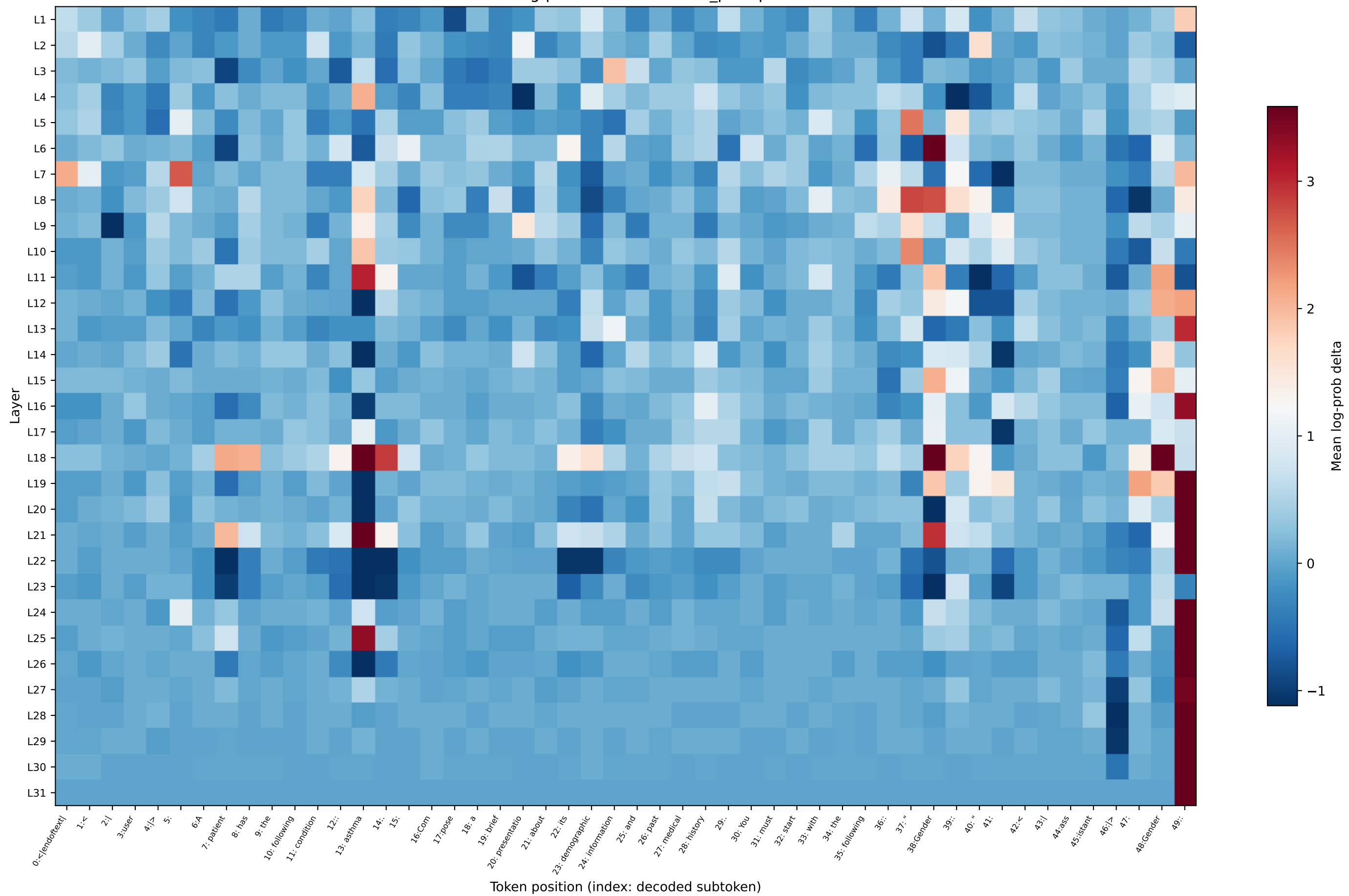
OLMo log-prob delta — asthma_prompt1
