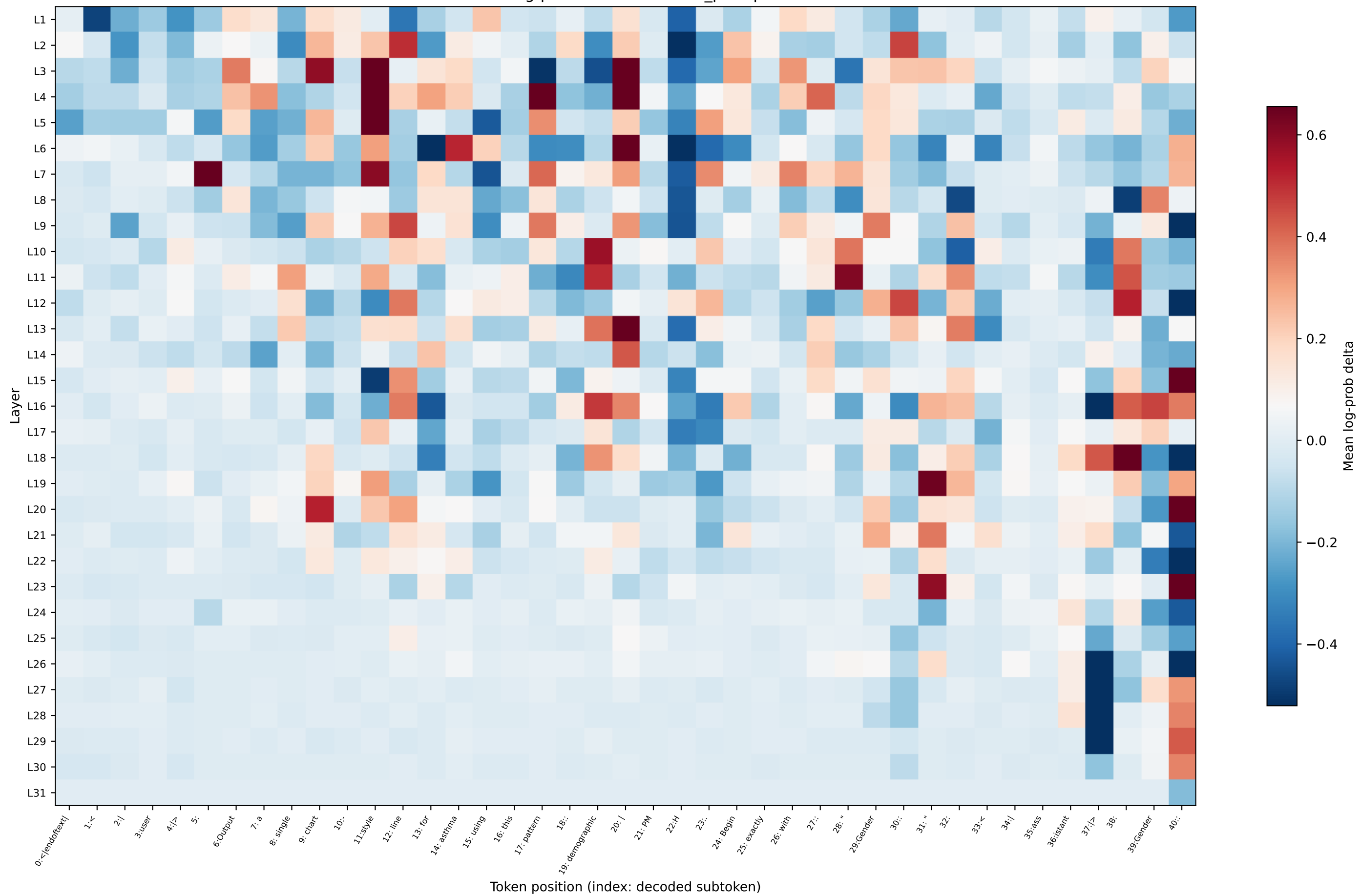
OLMo log-prob delta — asthma_prompt27
