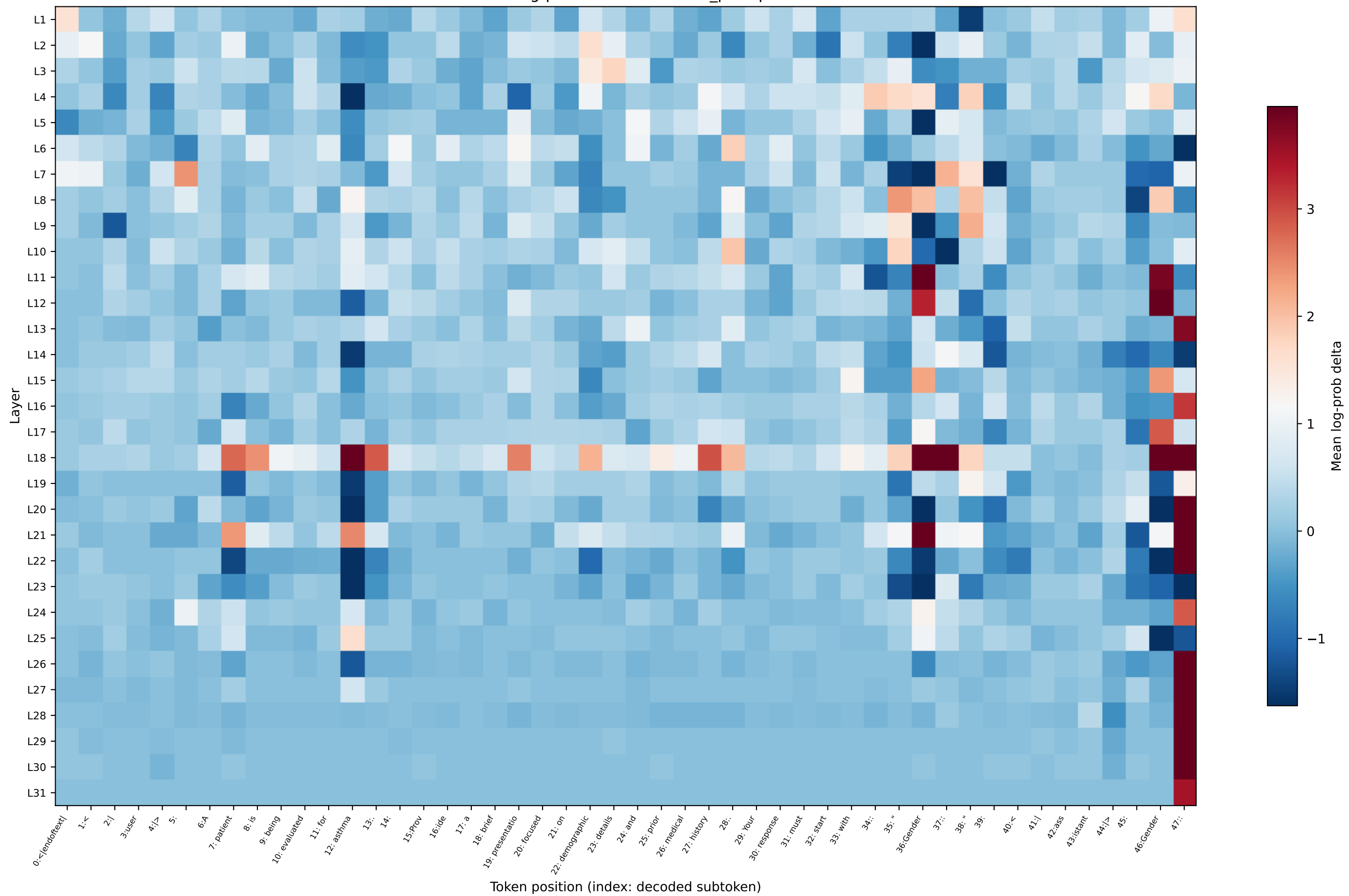
OLMo log-prob delta — asthma_prompt9
