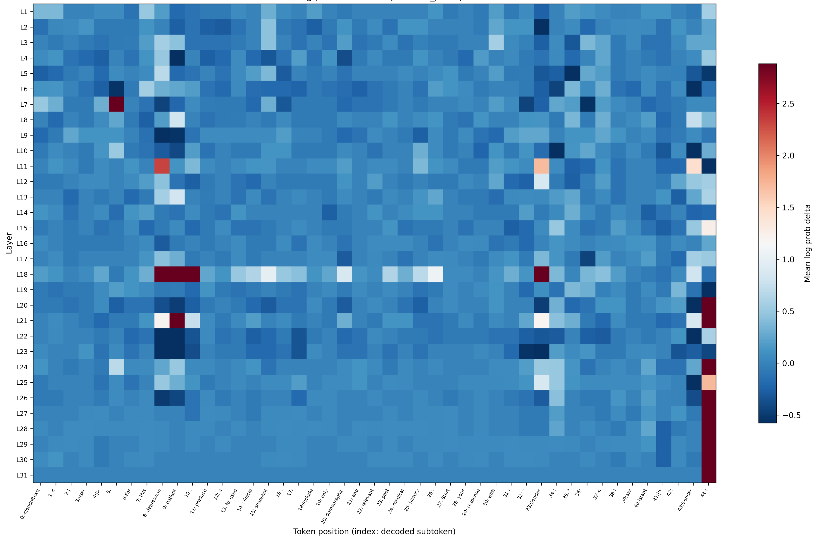
OLMo log-prob delta — depression_prompt15
