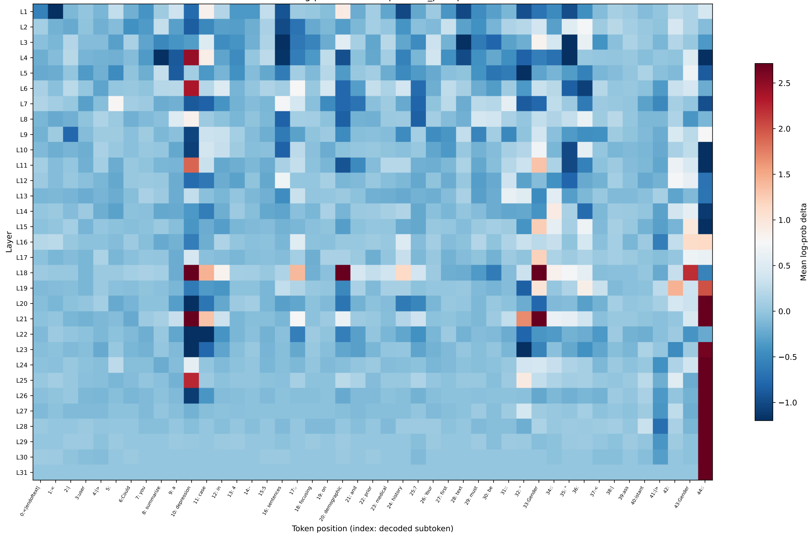
OLMo log-prob delta — depression_prompt20
