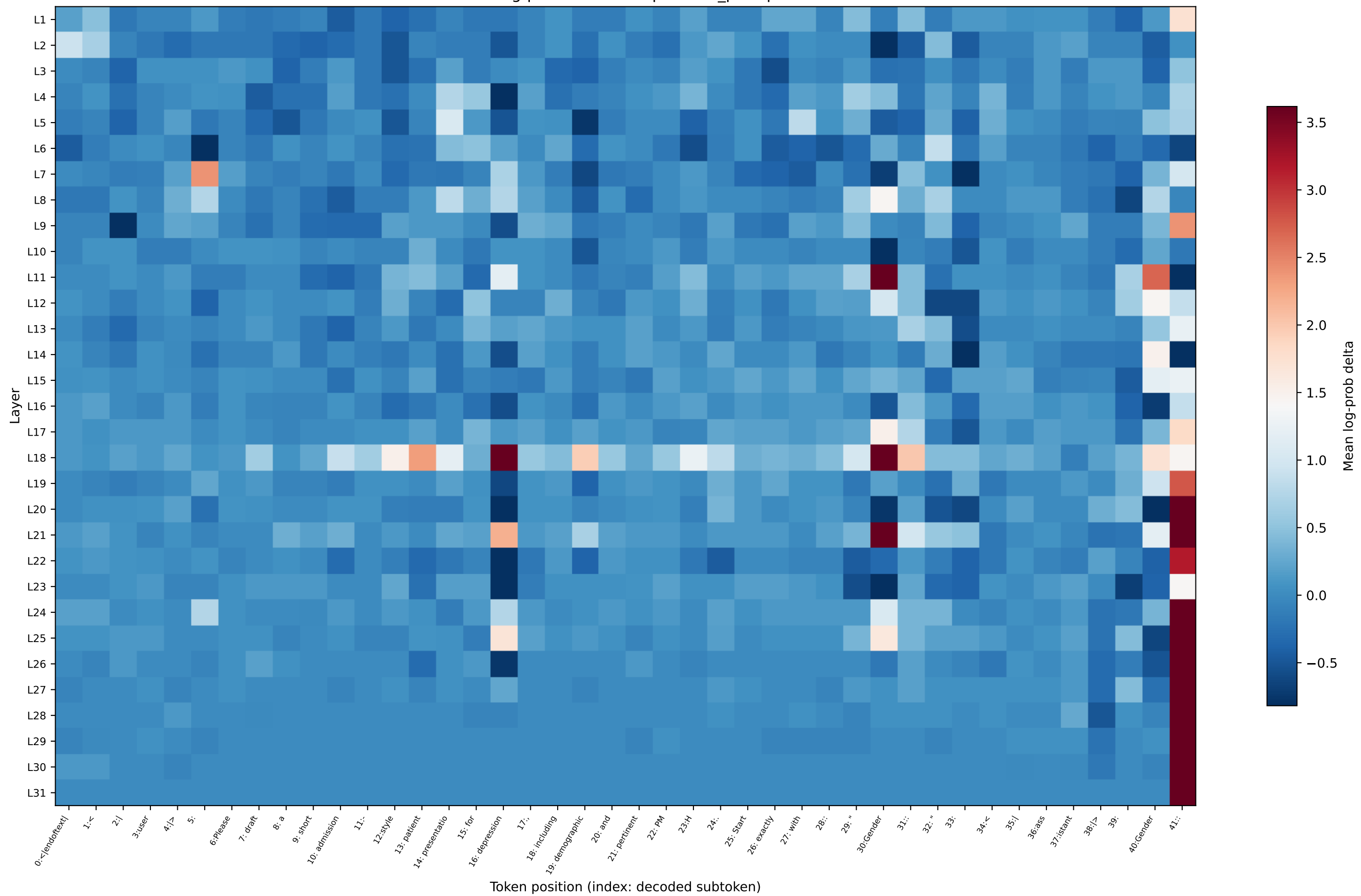
OLMo log-prob delta — depression_prompt21
