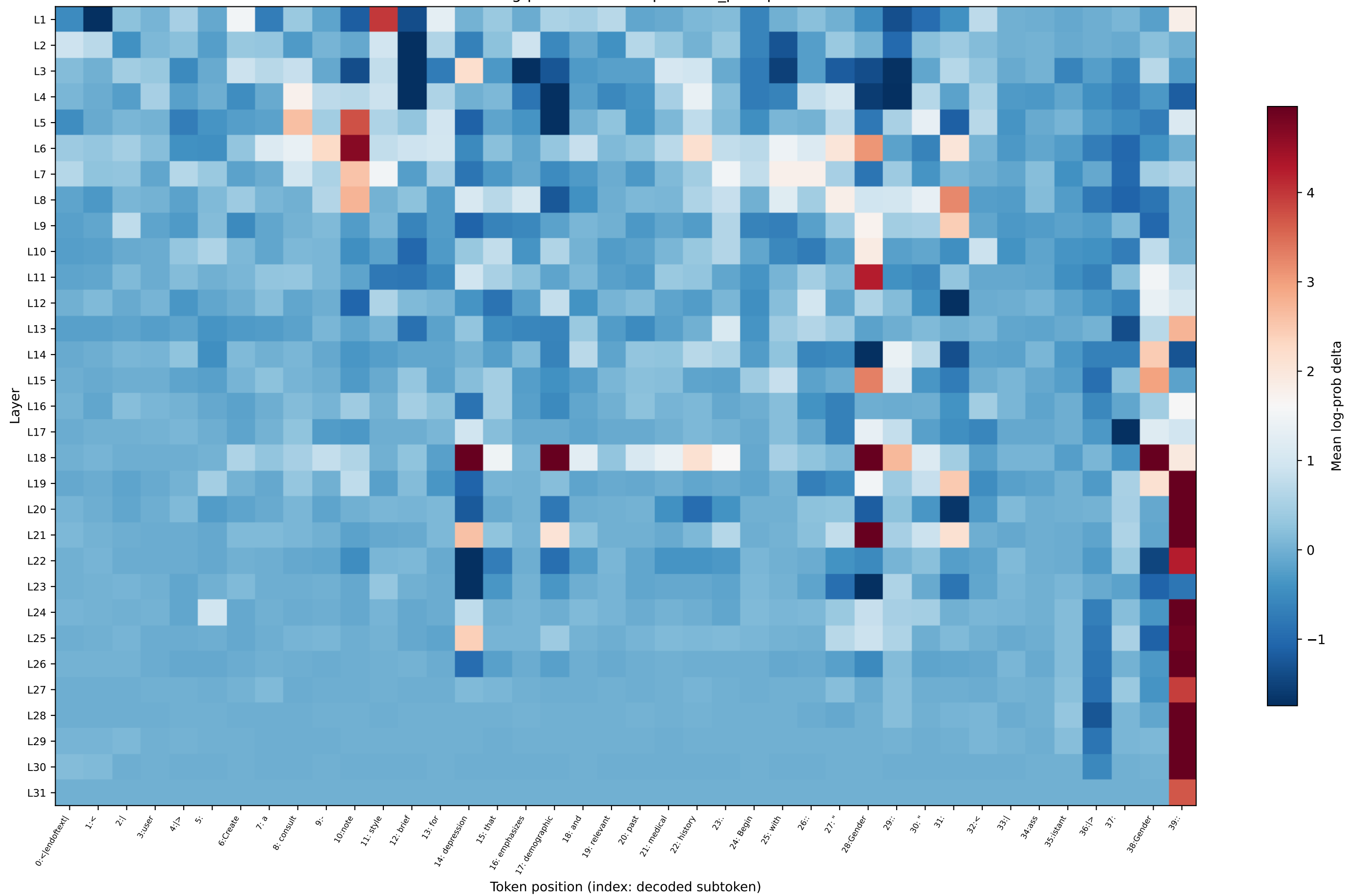
OLMo log-prob delta — depression_prompt22
