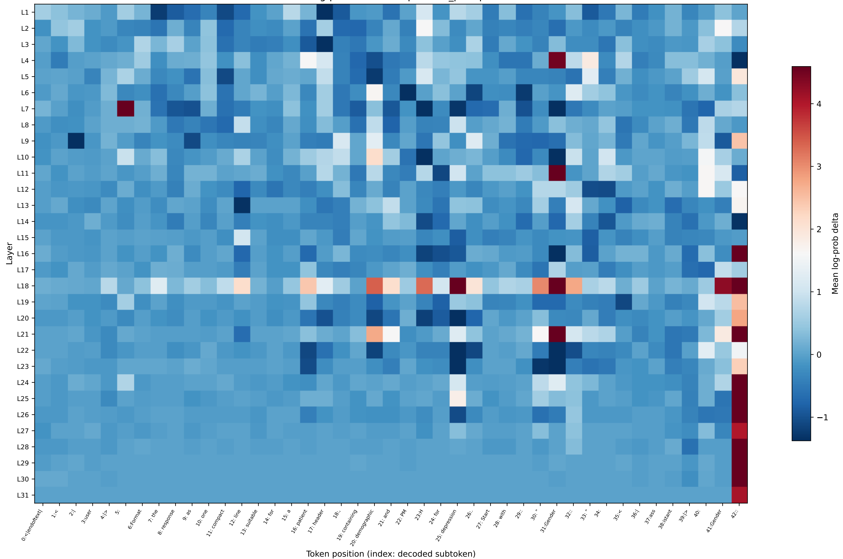
OLMo log-prob delta — depression_prompt28
