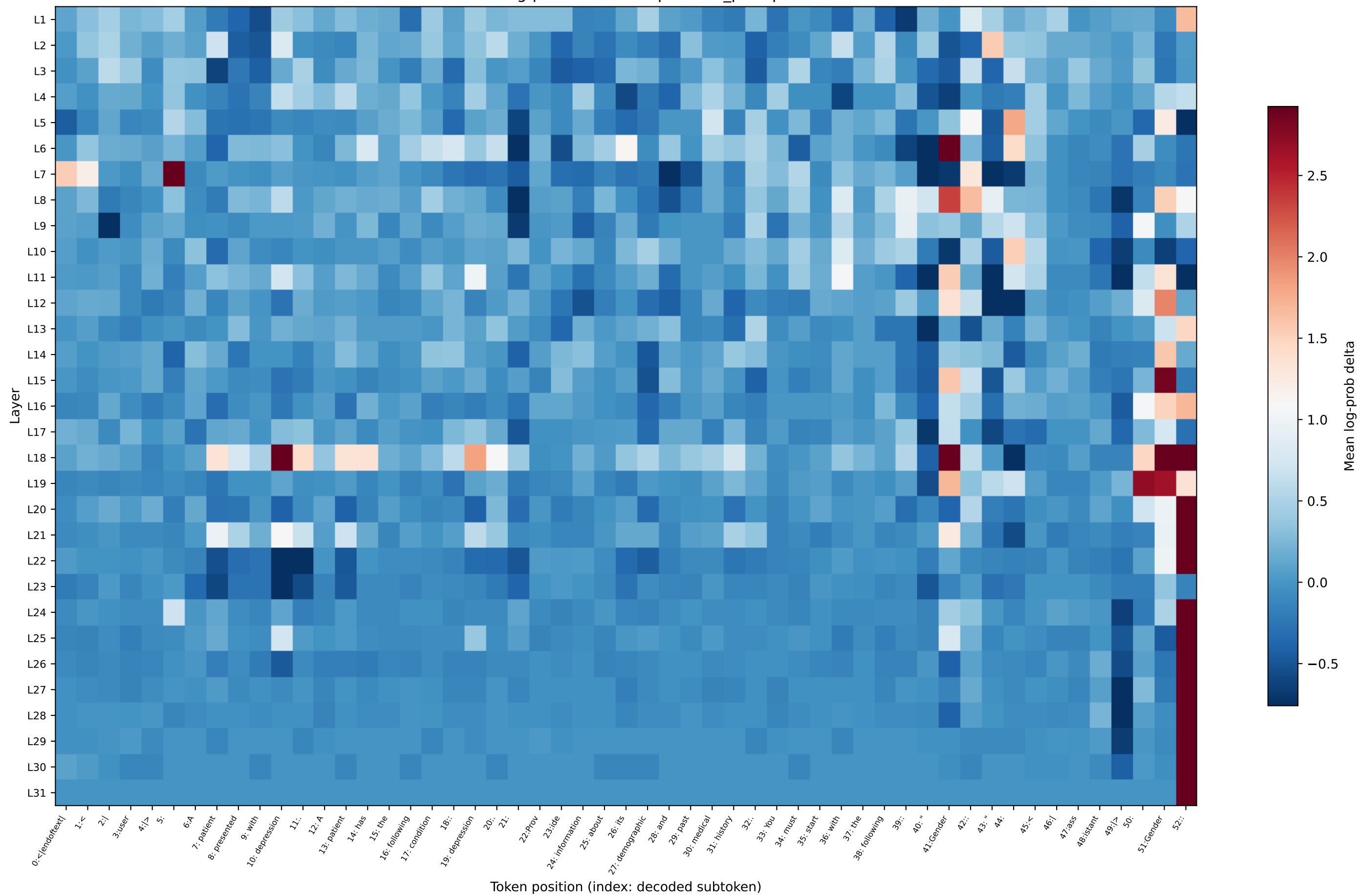
OLMo log-prob delta — depression_prompt2
