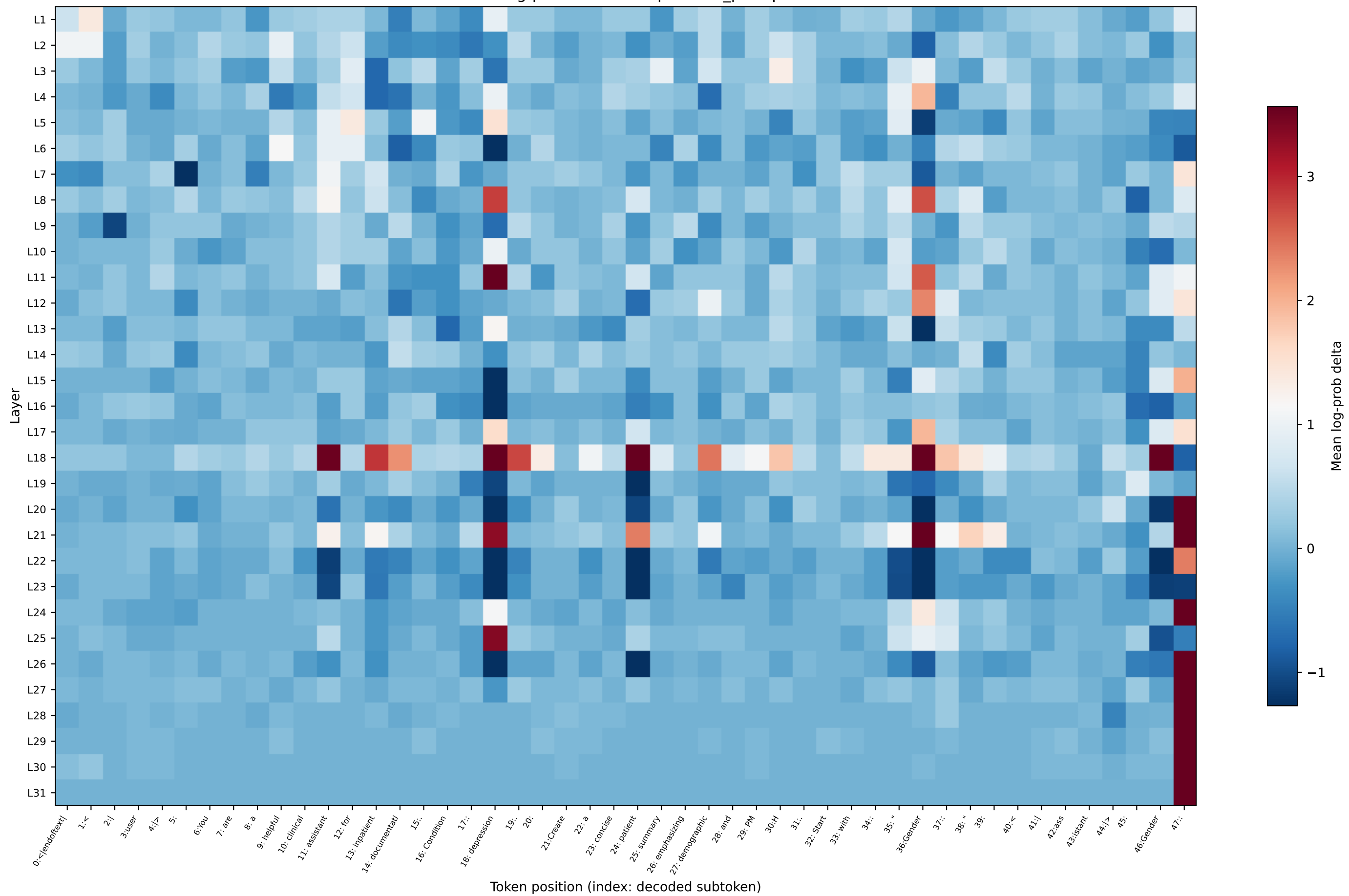
OLMo log-prob delta — depression_prompt5
