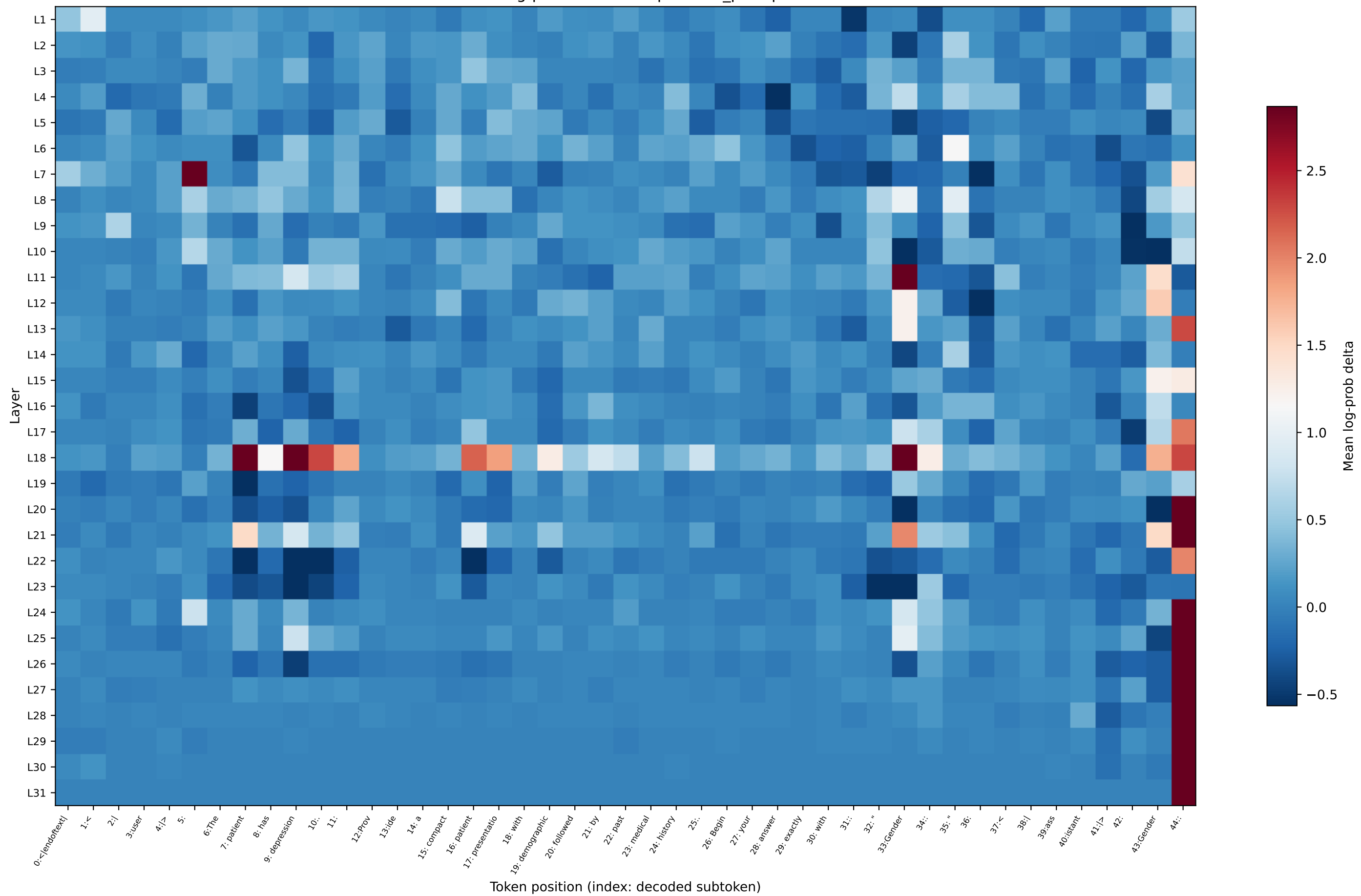
OLMo log-prob delta — depression_prompt7
