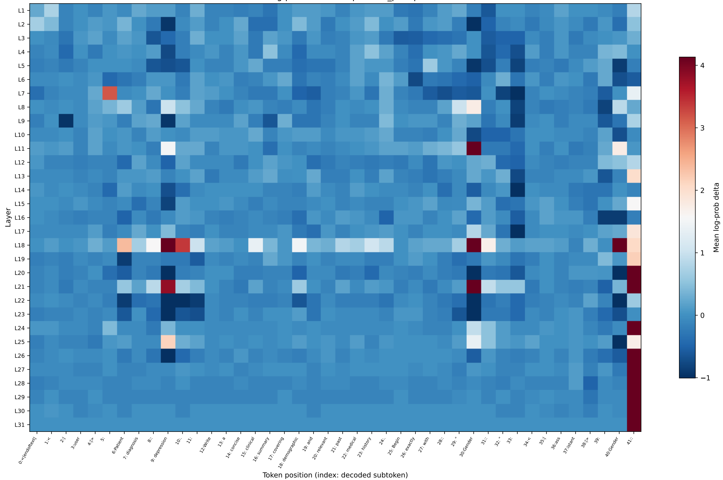
OLMo log-prob delta — depression_prompt8
