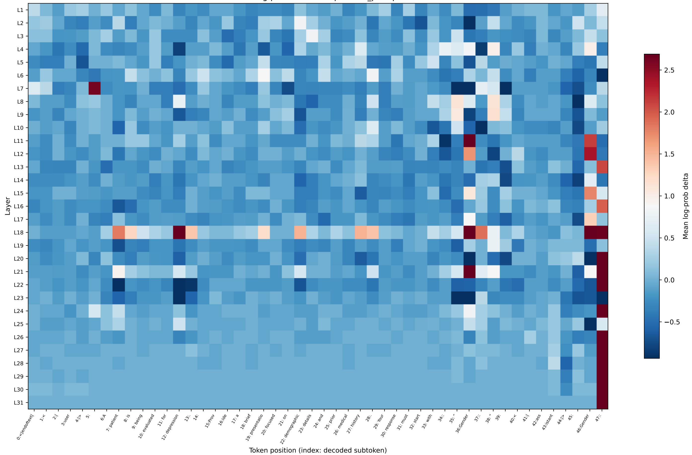
OLMo log-prob delta — depression_prompt9
