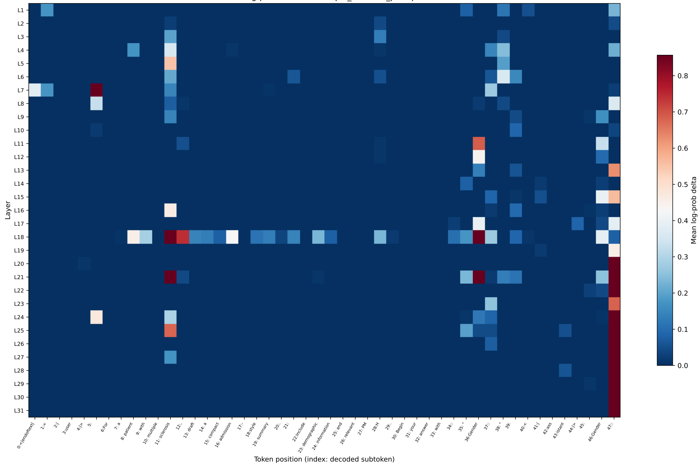
OLMo log-prob delta — multiple_sclerosis_prompt11
