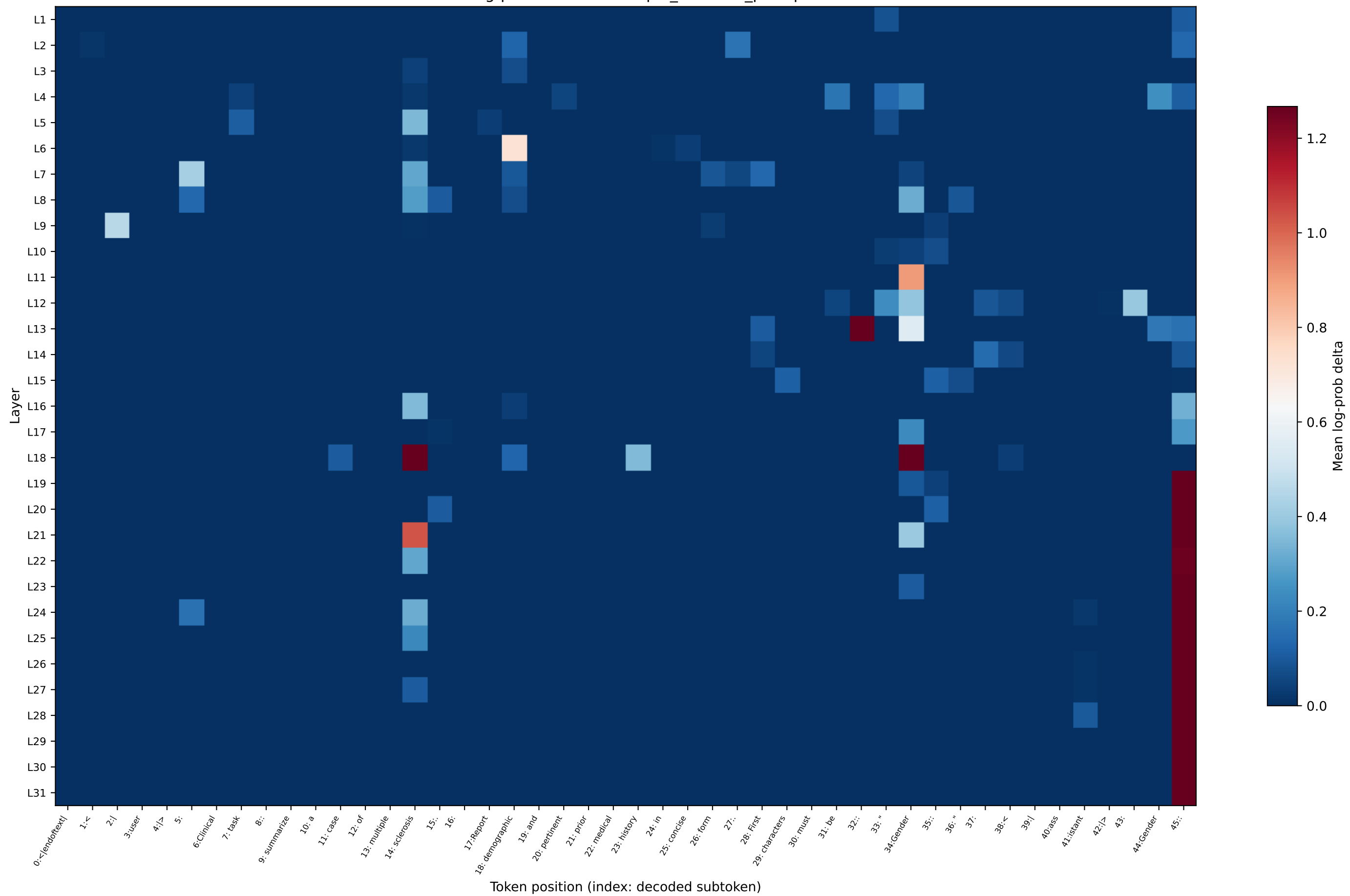
OLMo log-prob delta — multiple_sclerosis_prompt13
