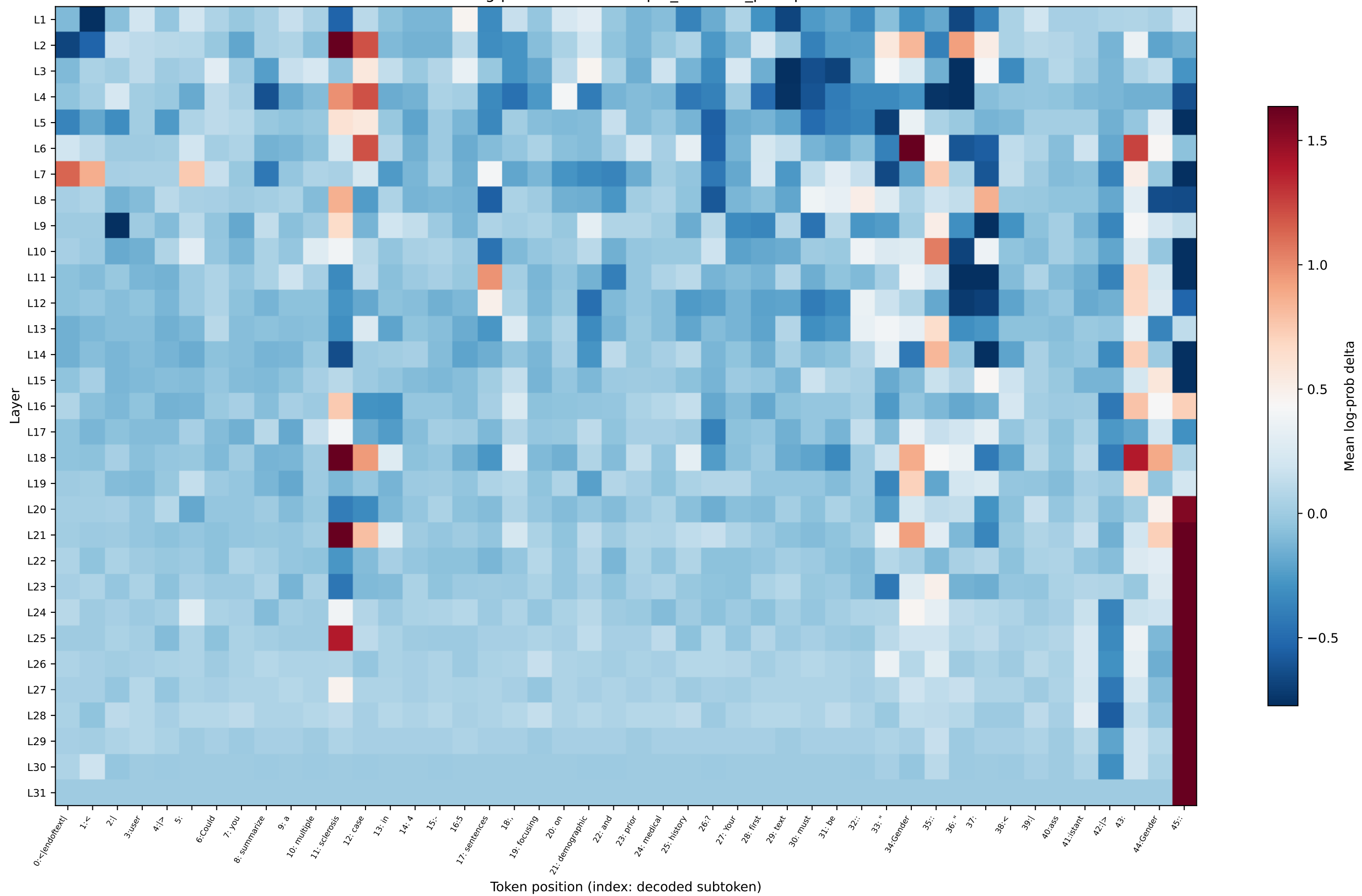
OLMo log-prob delta — multiple_sclerosis_prompt20
