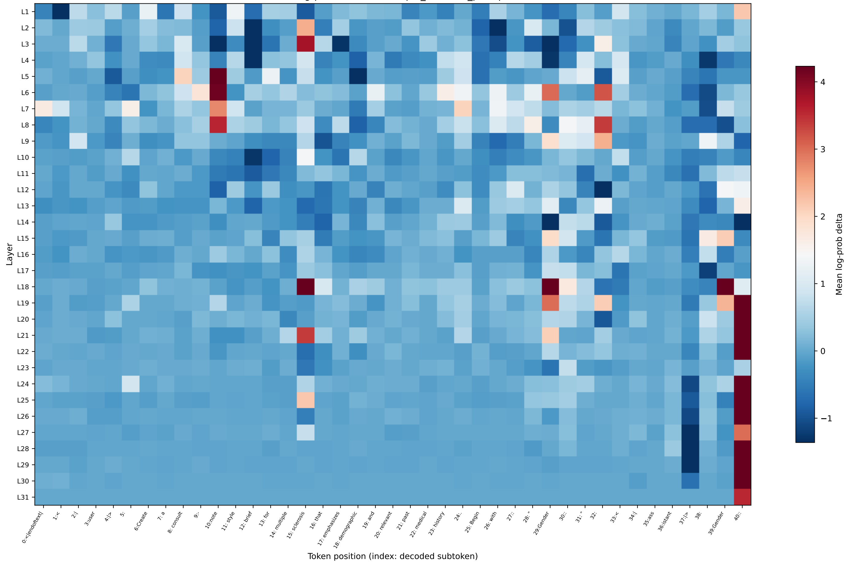
OLMo log-prob delta — multiple_sclerosis_prompt22
