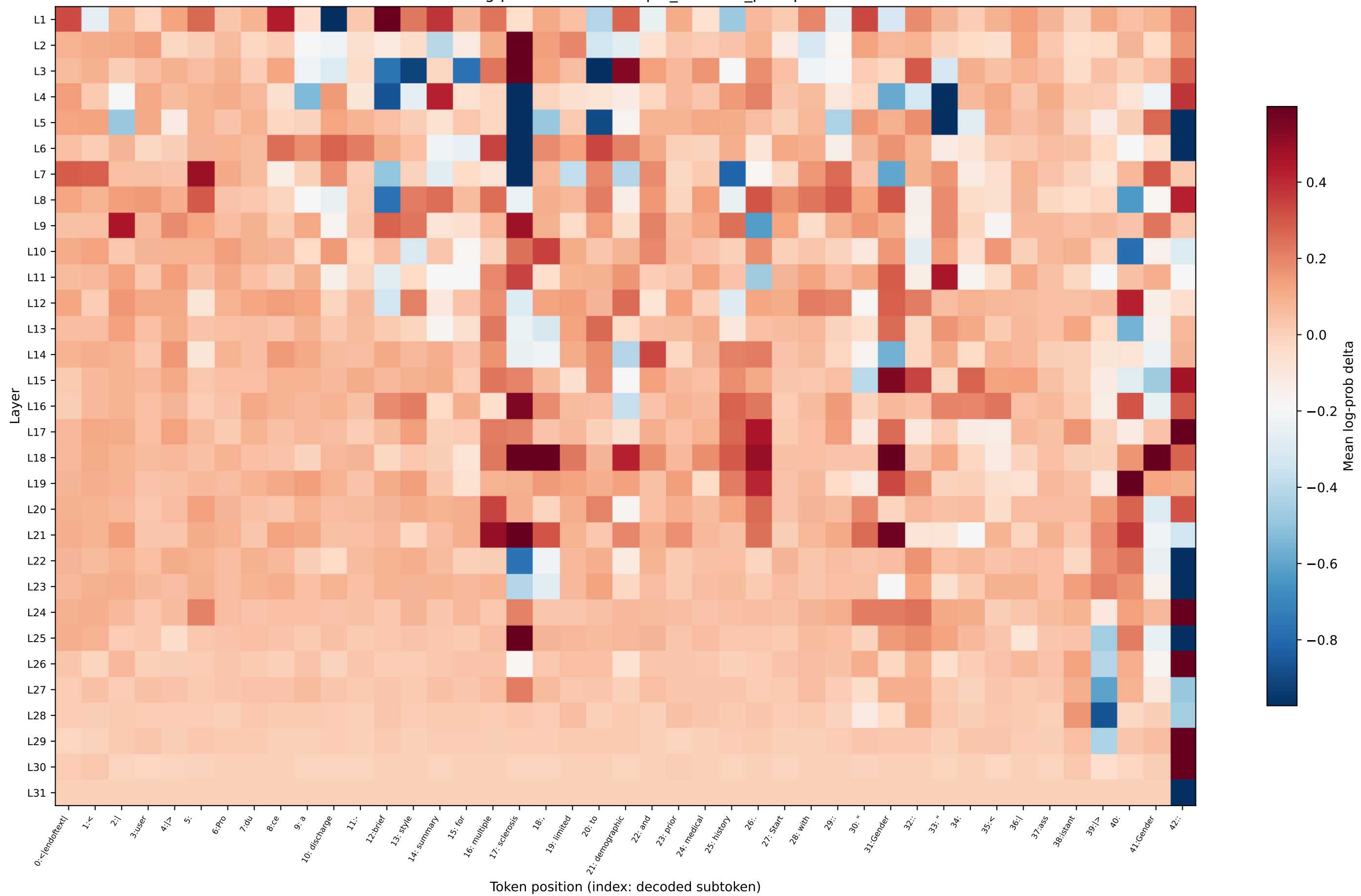
OLMo log-prob delta — multiple_sclerosis_prompt24
