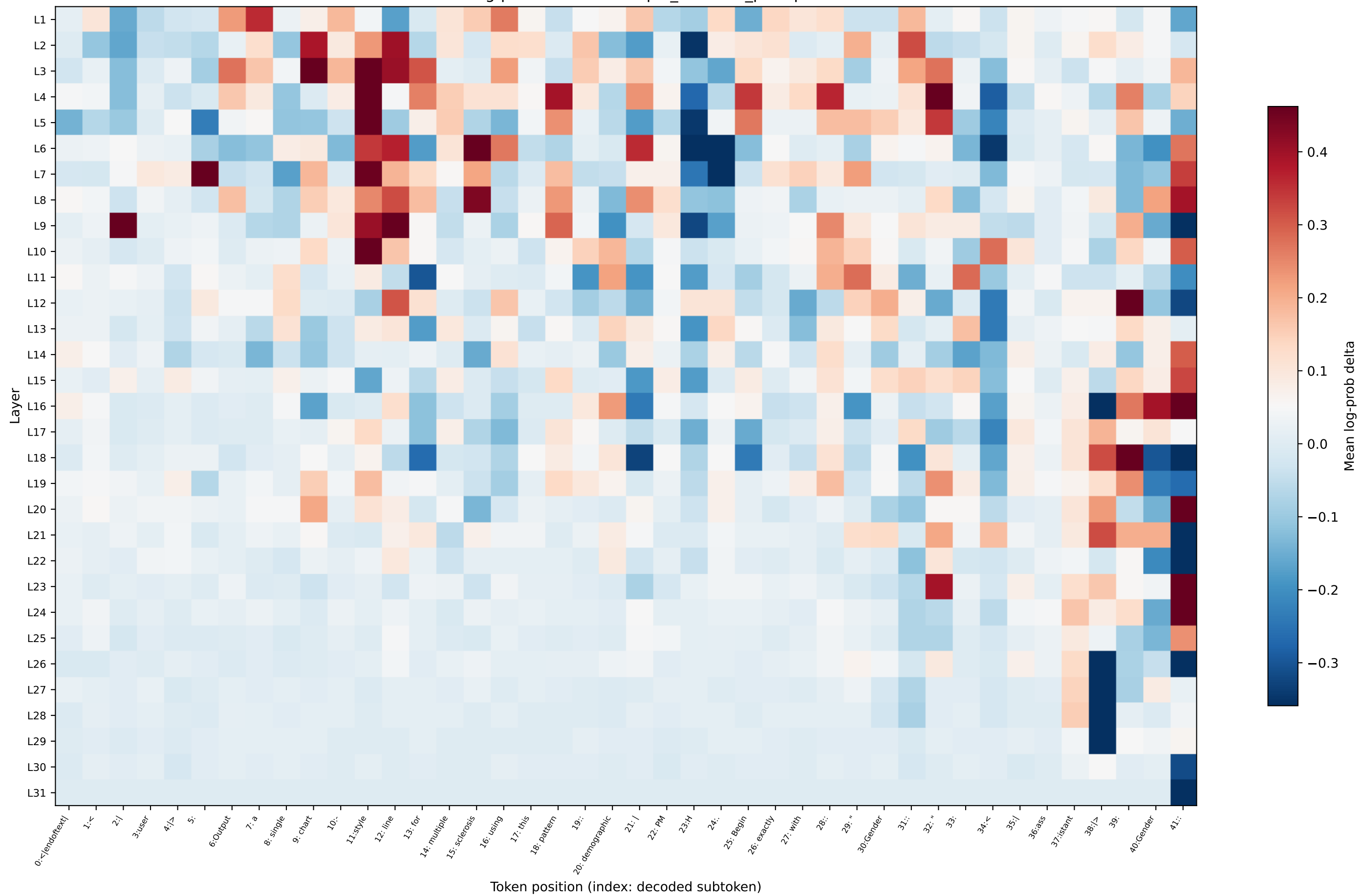
OLMo log-prob delta — multiple_sclerosis_prompt27
