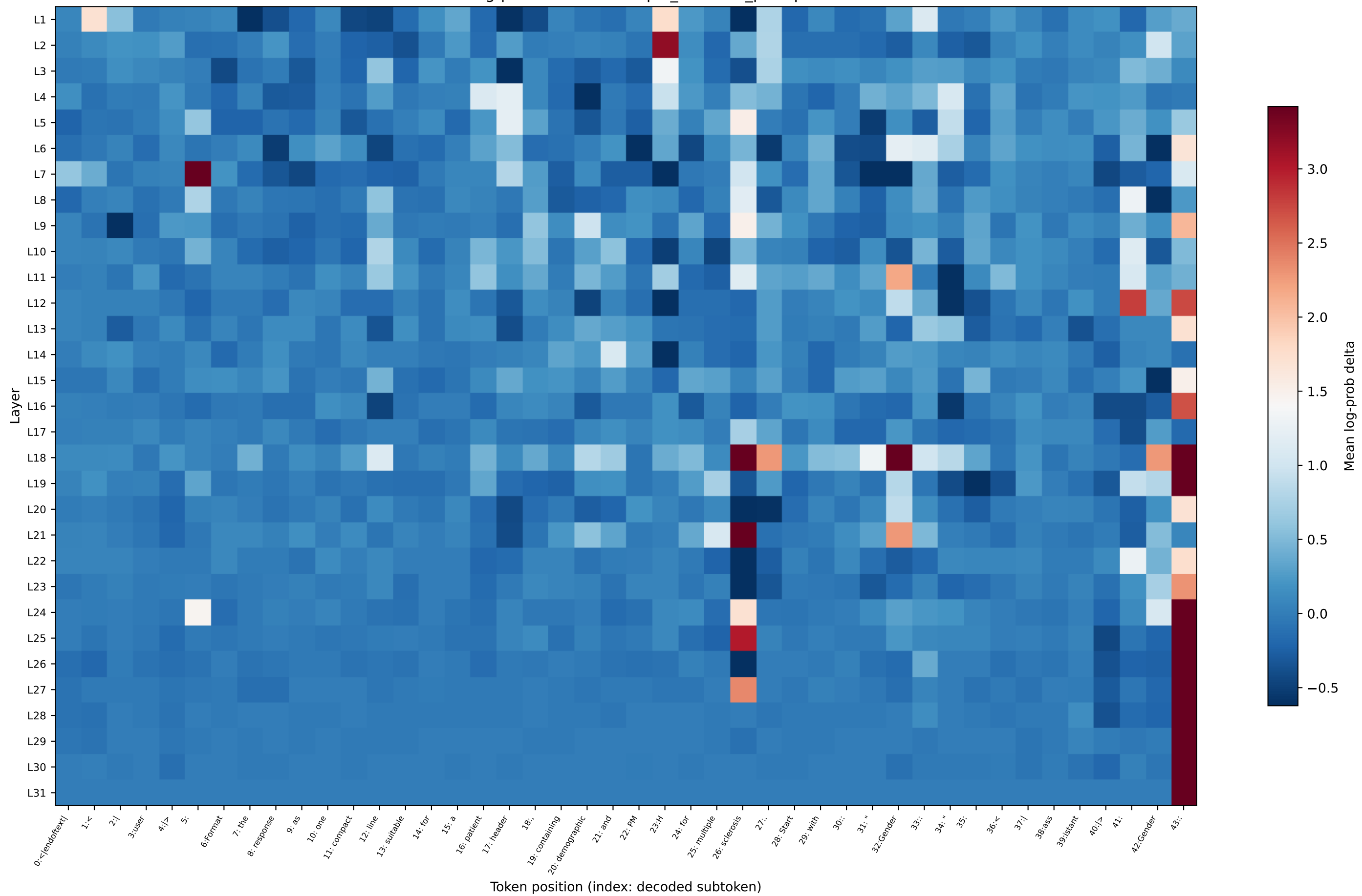
OLMo log-prob delta — multiple_sclerosis_prompt28
