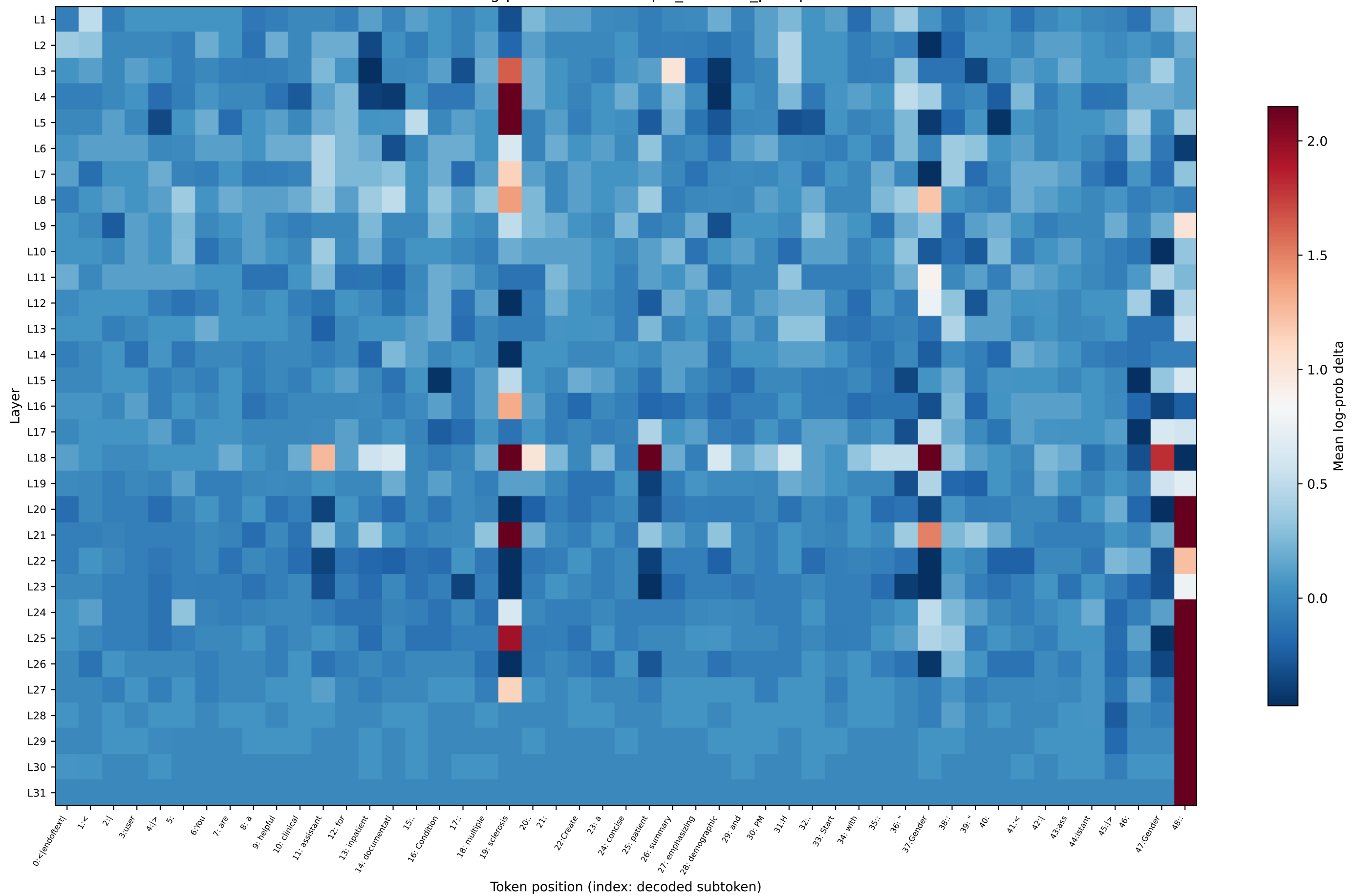
OLMo log-prob delta — multiple_sclerosis_prompt5
