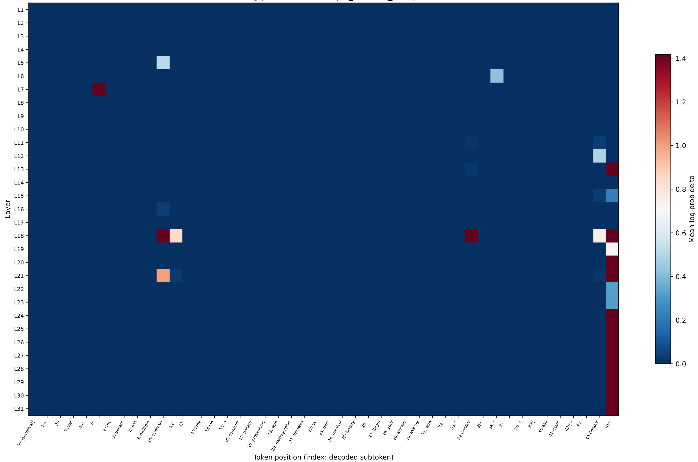
OLMo log-prob delta — multiple_sclerosis_prompt7
