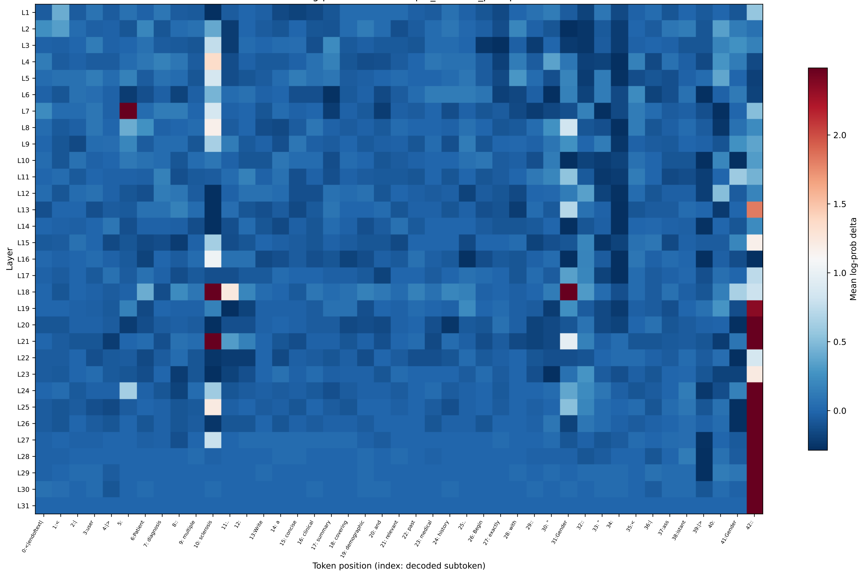
OLMo log-prob delta — multiple_sclerosis_prompt8
