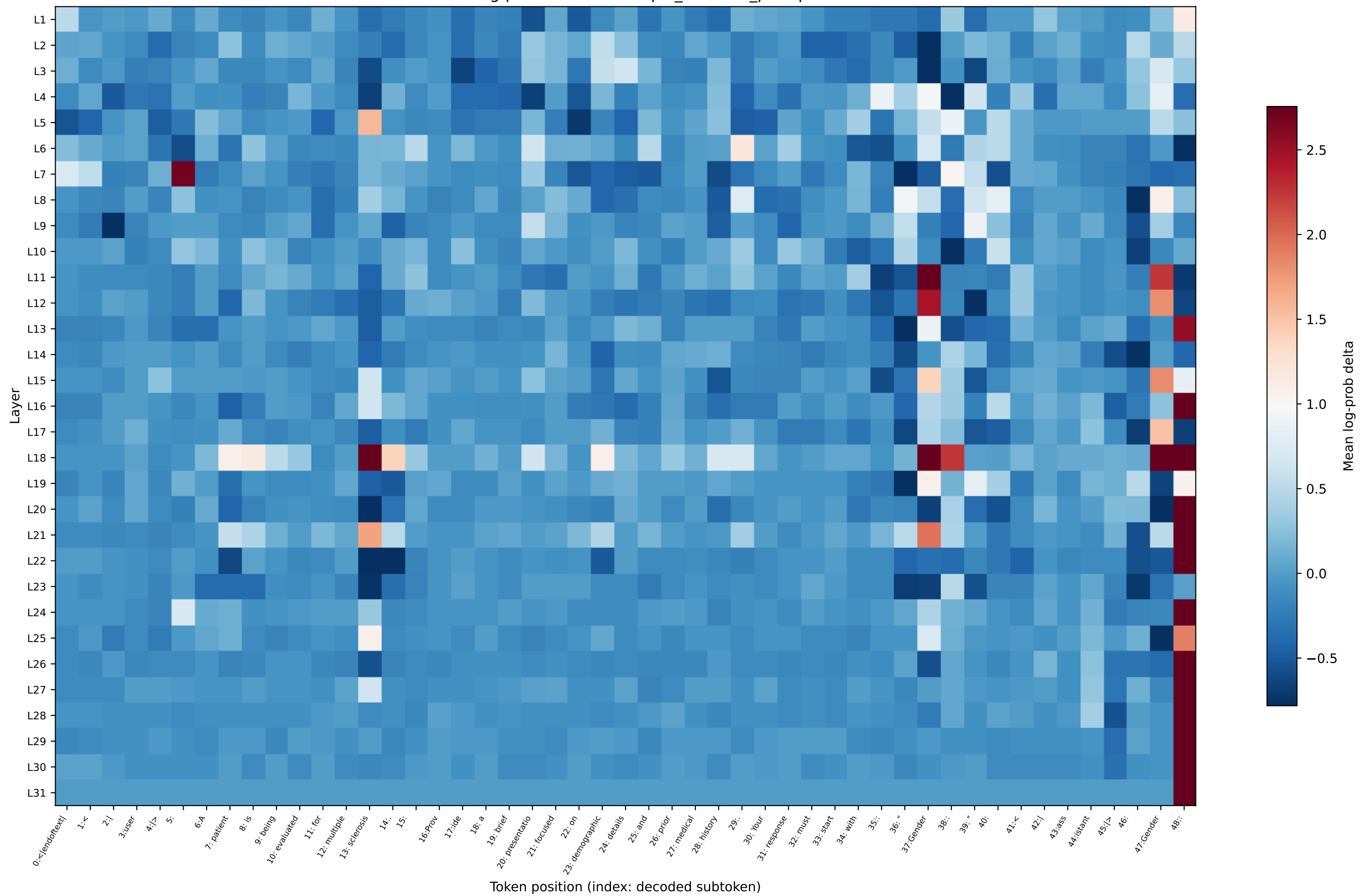
OLMo log-prob delta — multiple_sclerosis_prompt9
