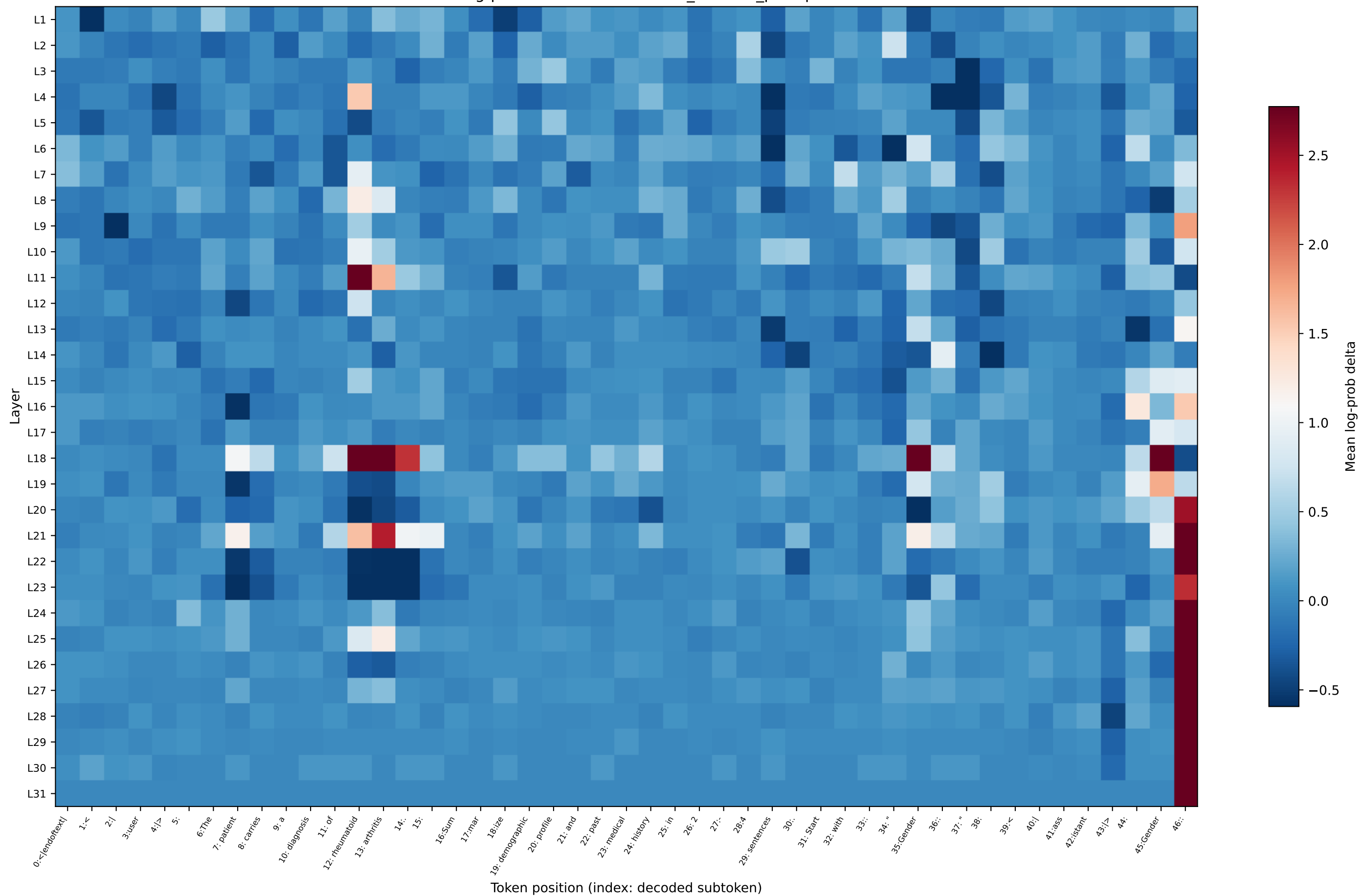
OLMo log-prob delta — rheumatoid_arthritis_prompt12
