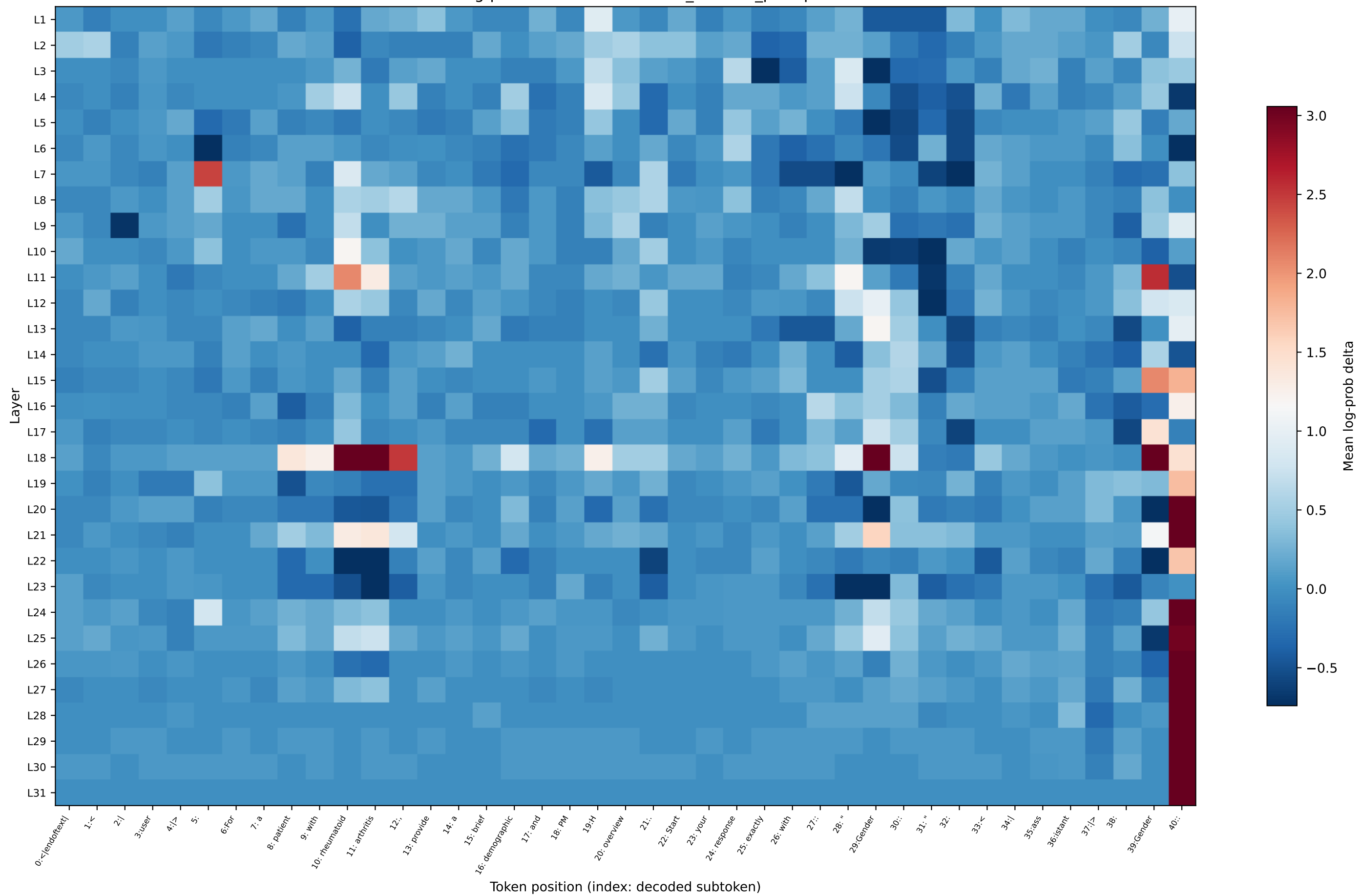
OLMo log-prob delta — rheumatoid_arthritis_prompt19
