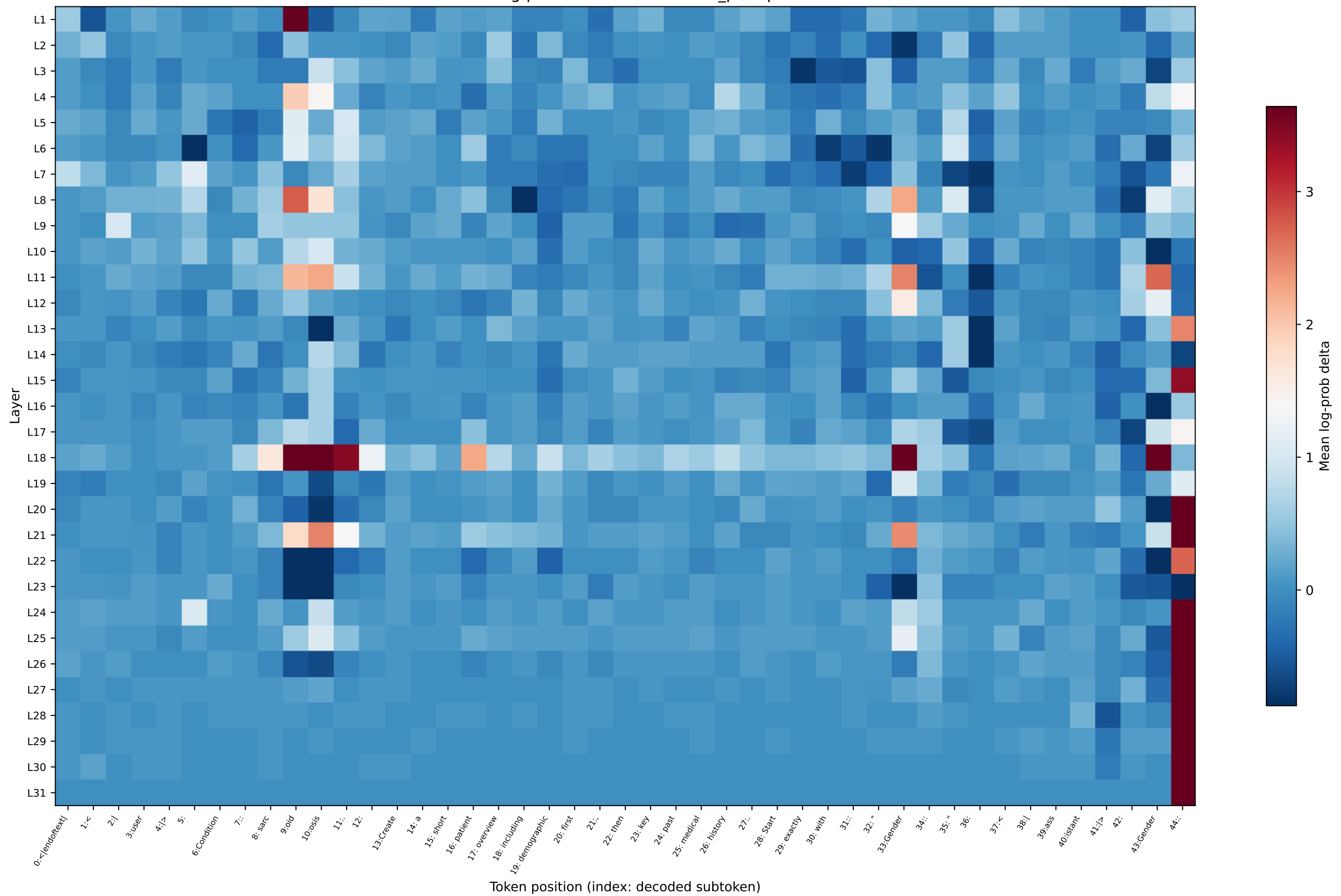
OLMo log-prob delta — sarcoidosis_prompt10
