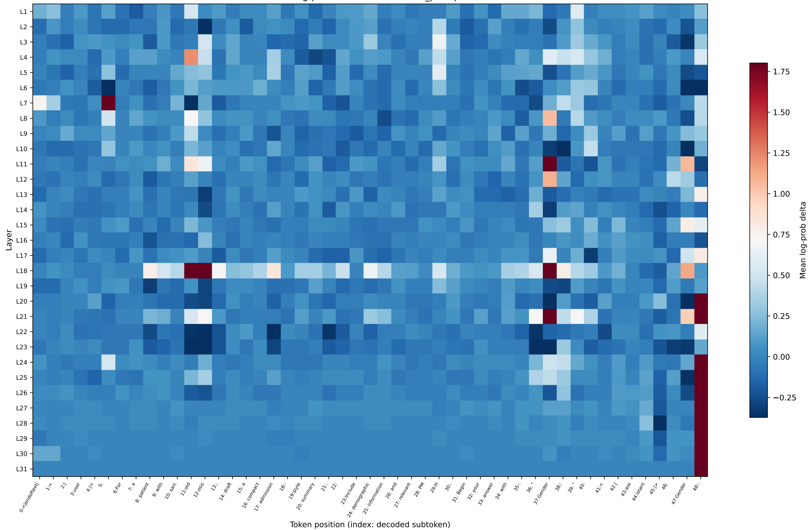
OLMo log-prob delta — sarcoidosis_prompt11
