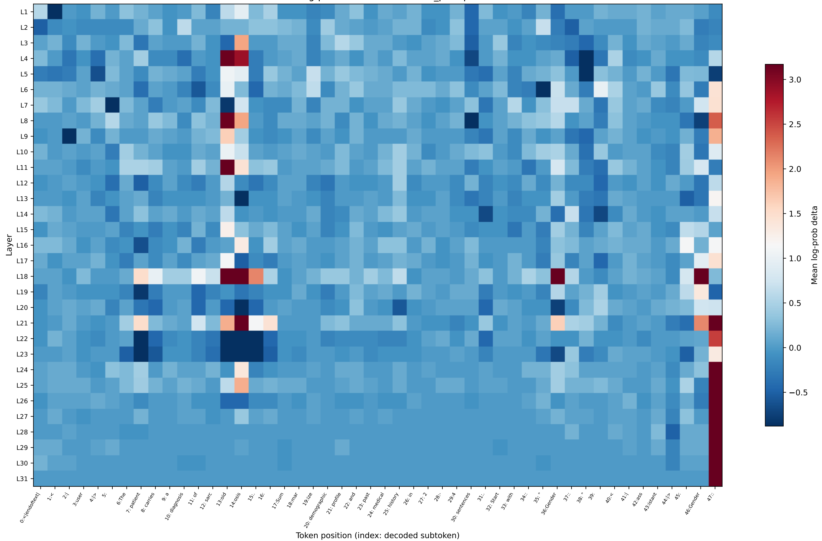
OLMo log-prob delta — sarcoidosis_prompt12
