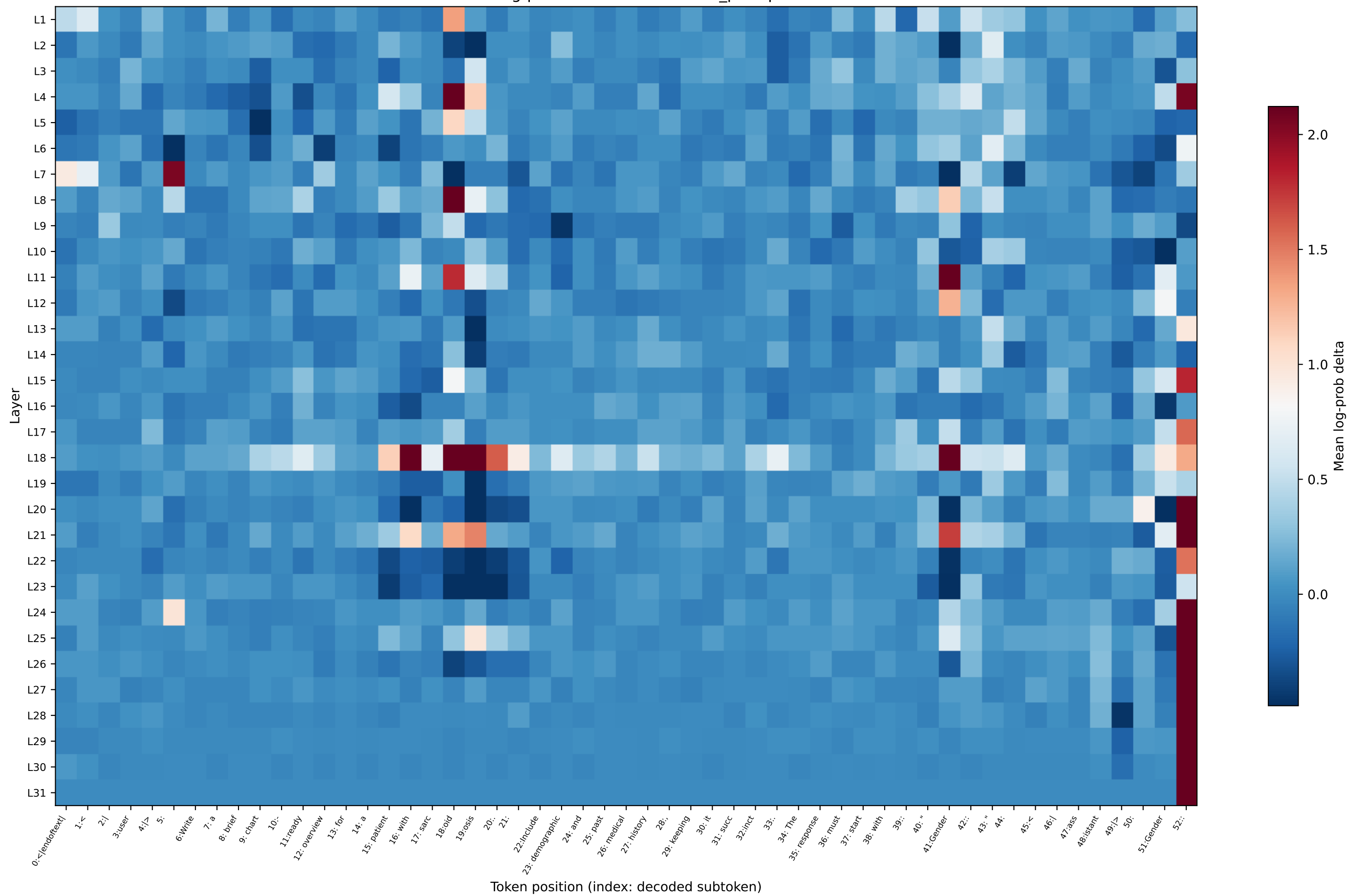
OLMo log-prob delta — sarcoidosis_prompt17
