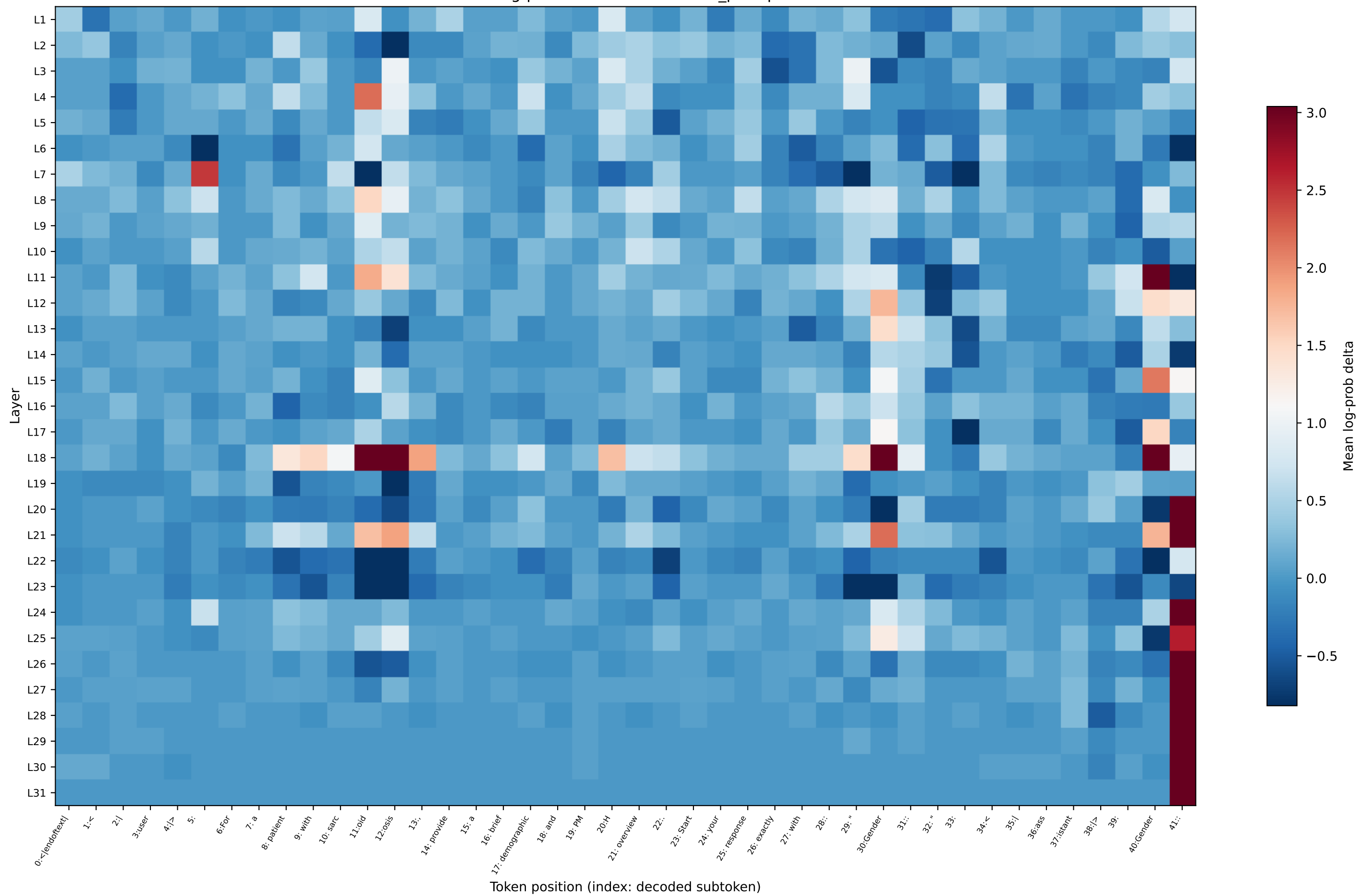
OLMo log-prob delta — sarcoidosis_prompt19
