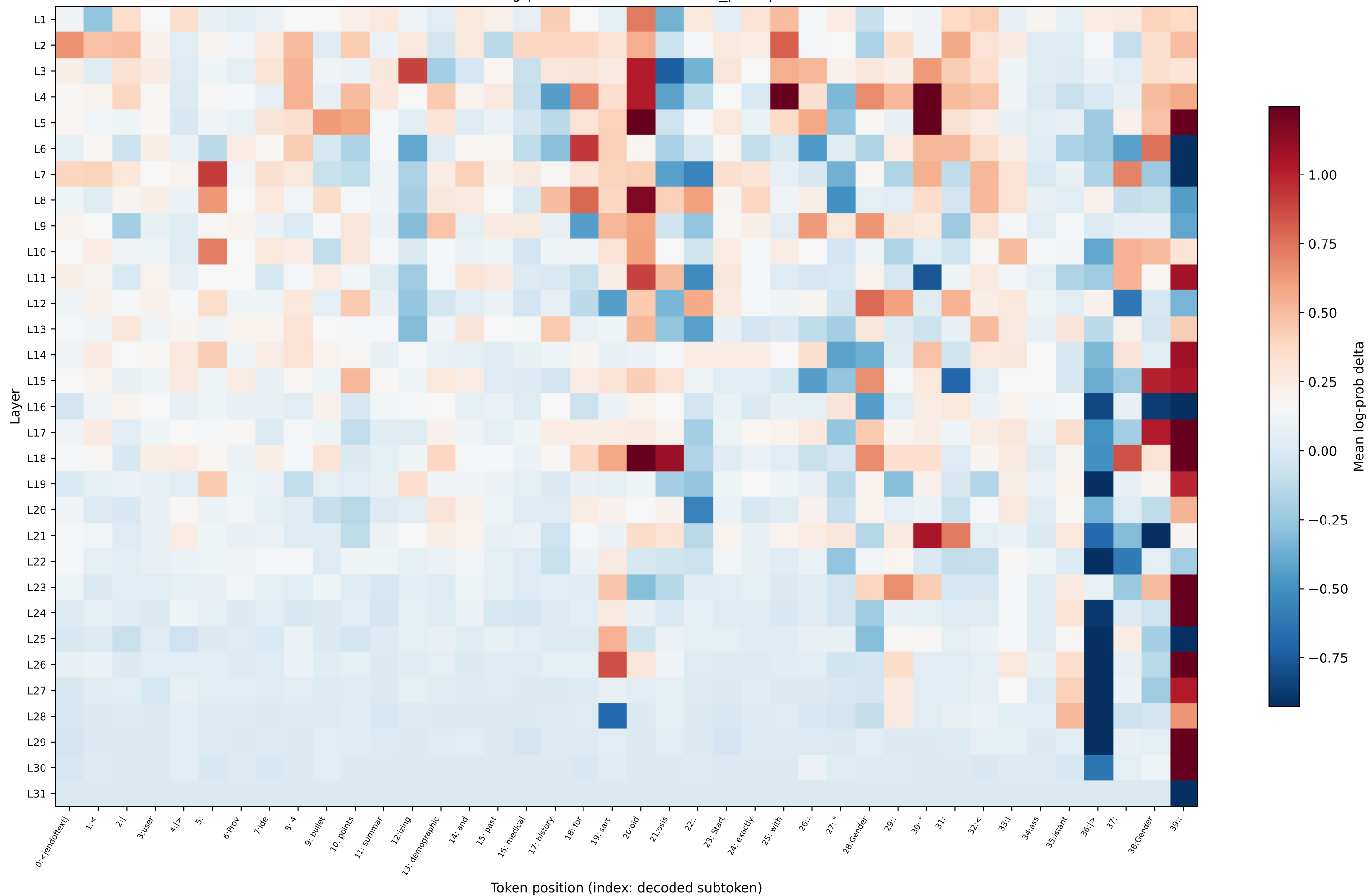
OLMo log-prob delta — sarcoidosis_prompt26
