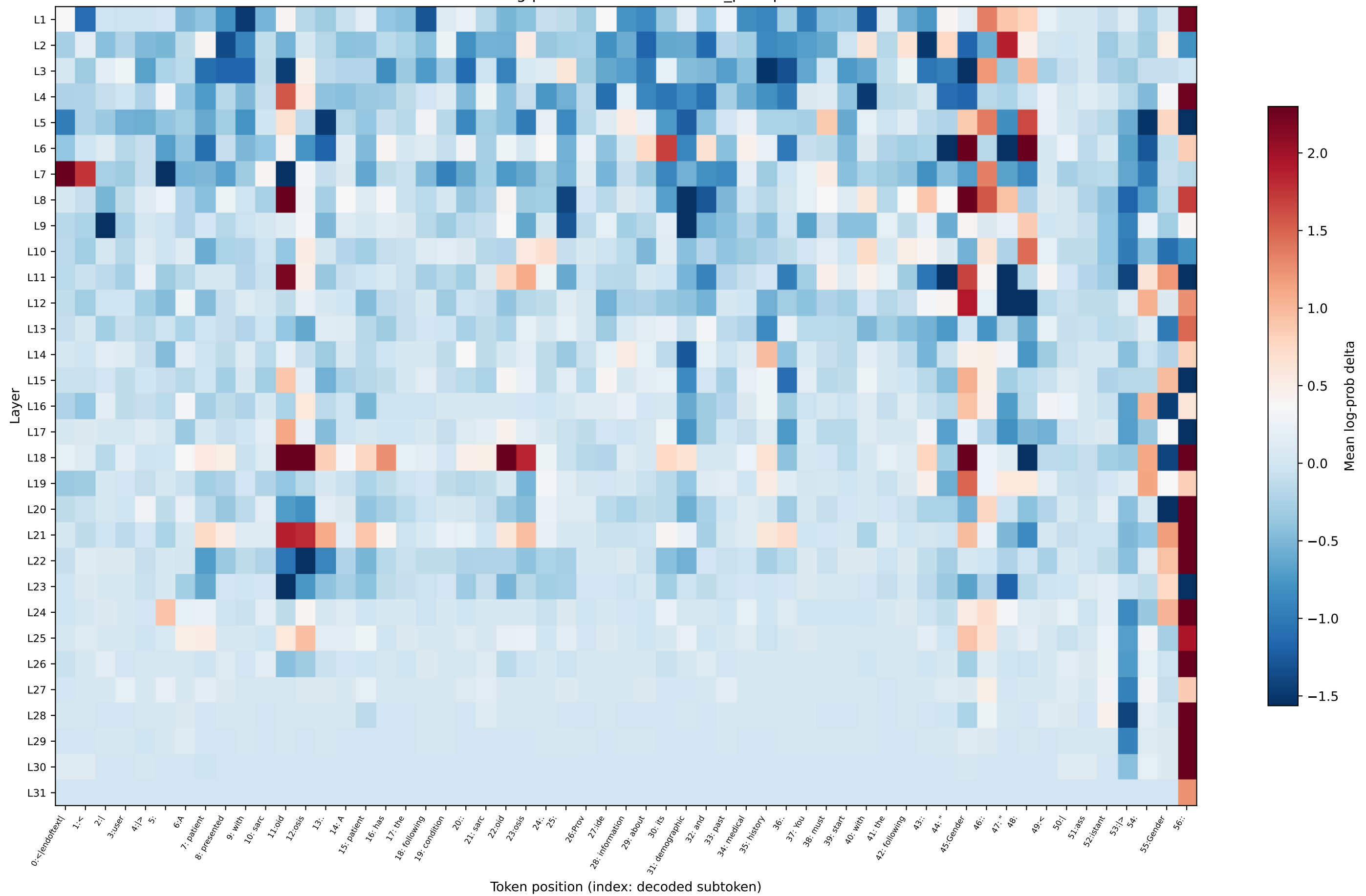
OLMo log-prob delta — sarcoidosis_prompt2
