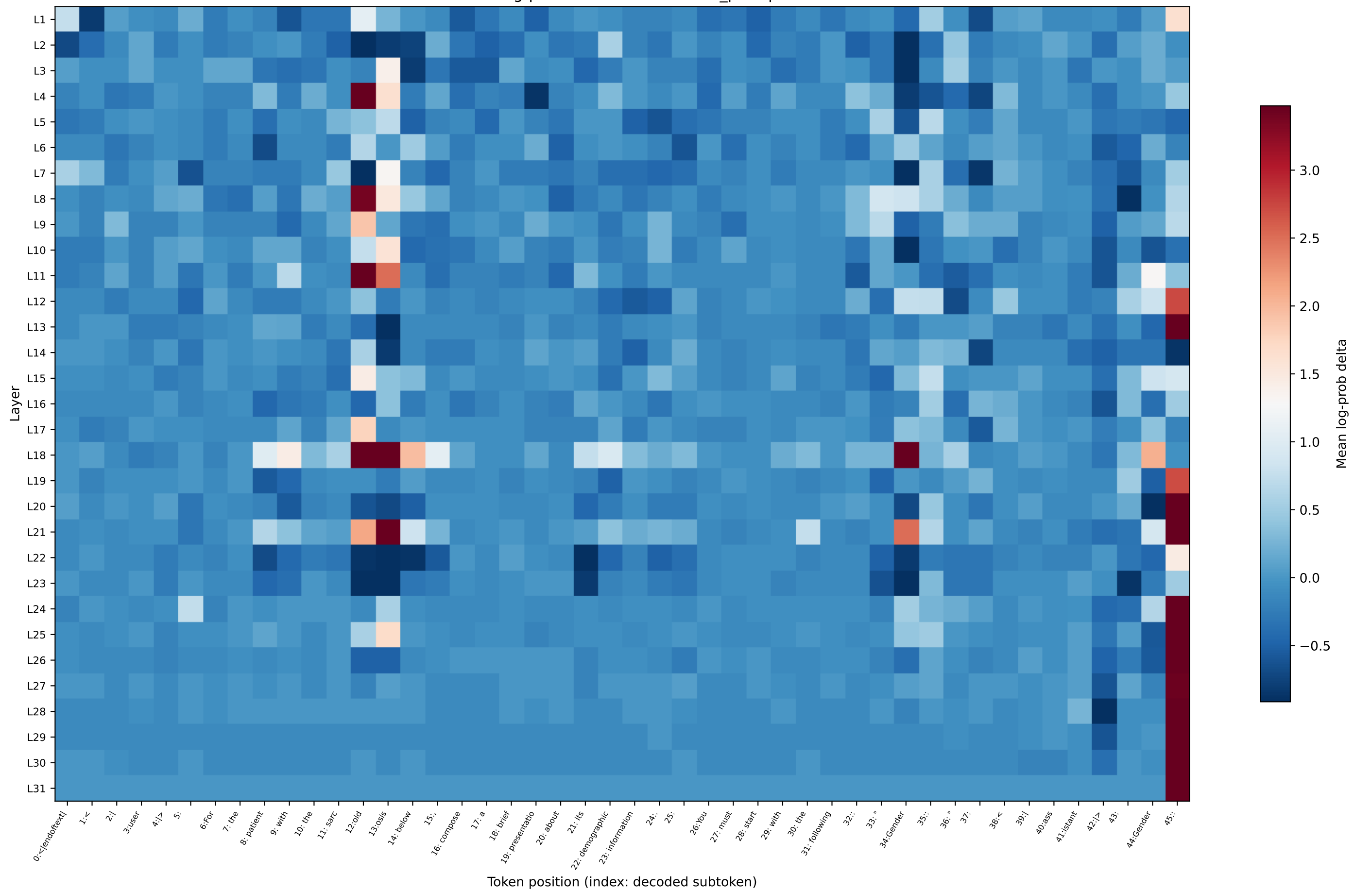
OLMo log-prob delta — sarcoidosis_prompt3
