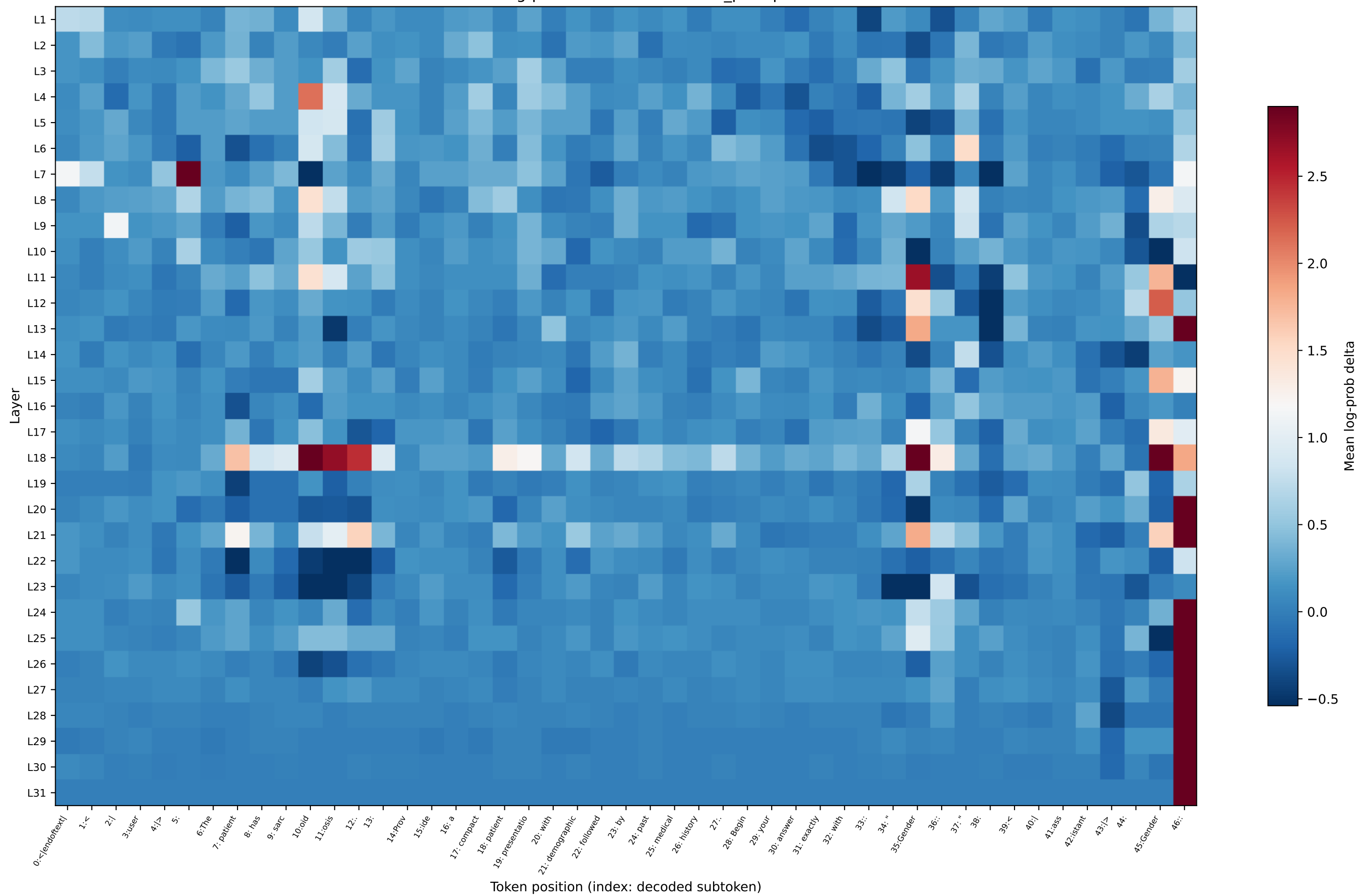
OLMo log-prob delta — sarcoidosis_prompt7
