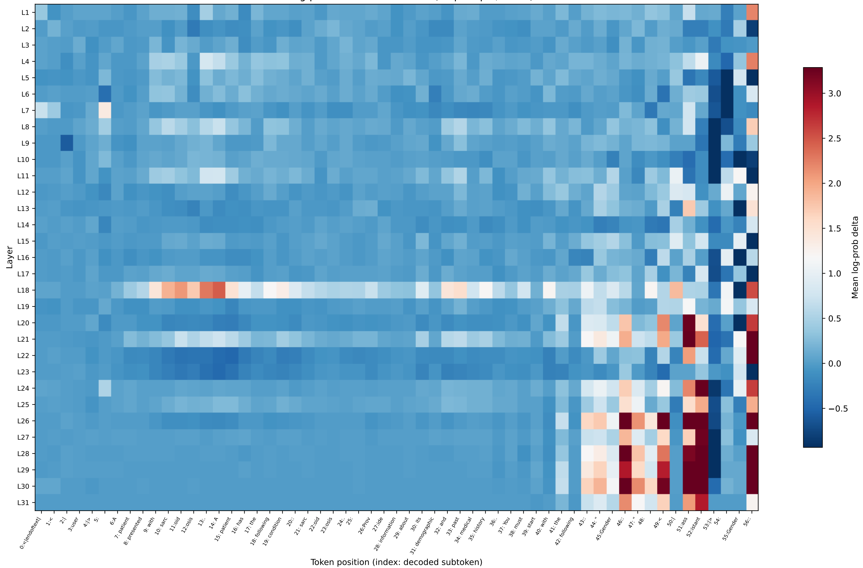
OLMo log-prob delta — sarcoidosis (31 prompts, mean)
