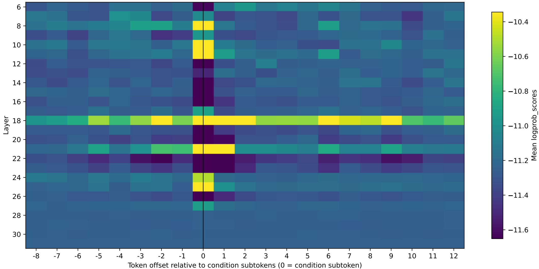
OLMo asthma, 31 prompts: condition-aligned mean logprob_scores
