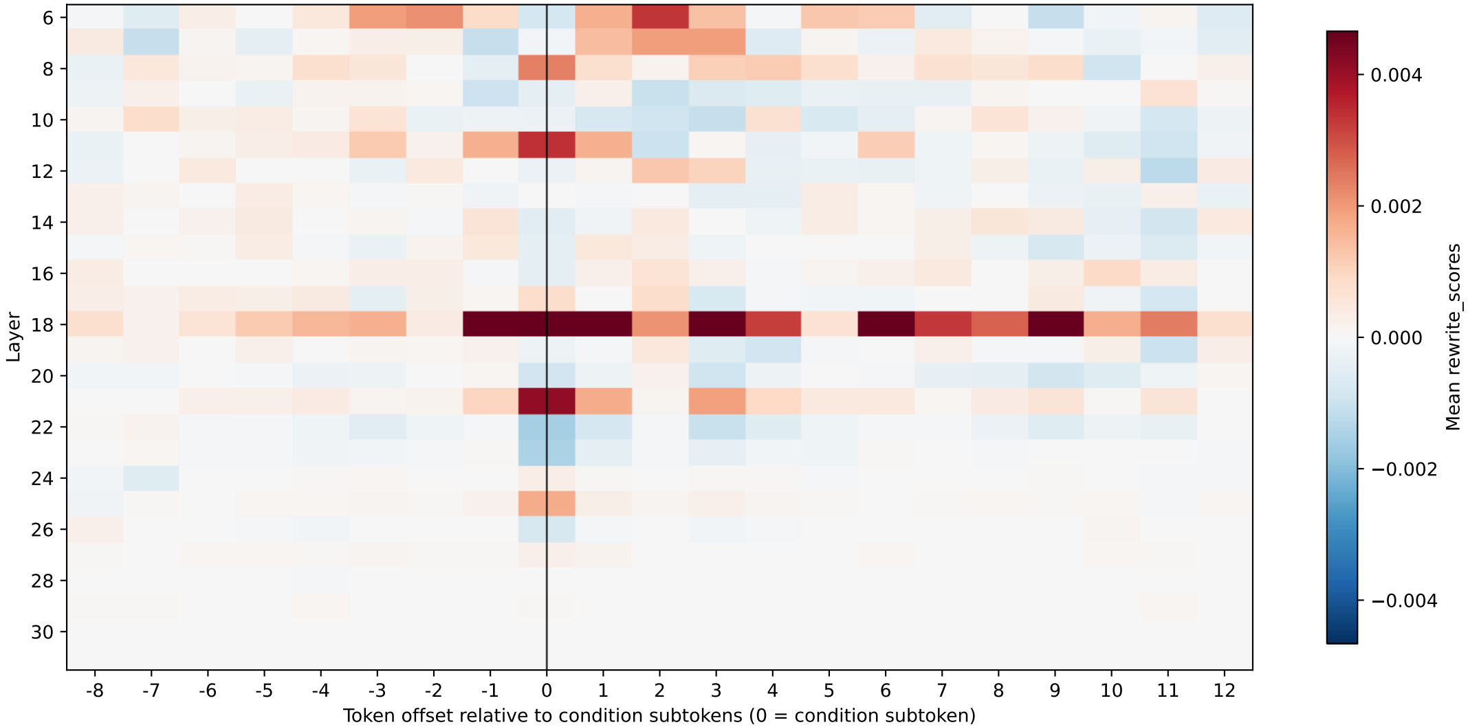
OLMo all 155 units: condition-aligned mean rewrite scores
