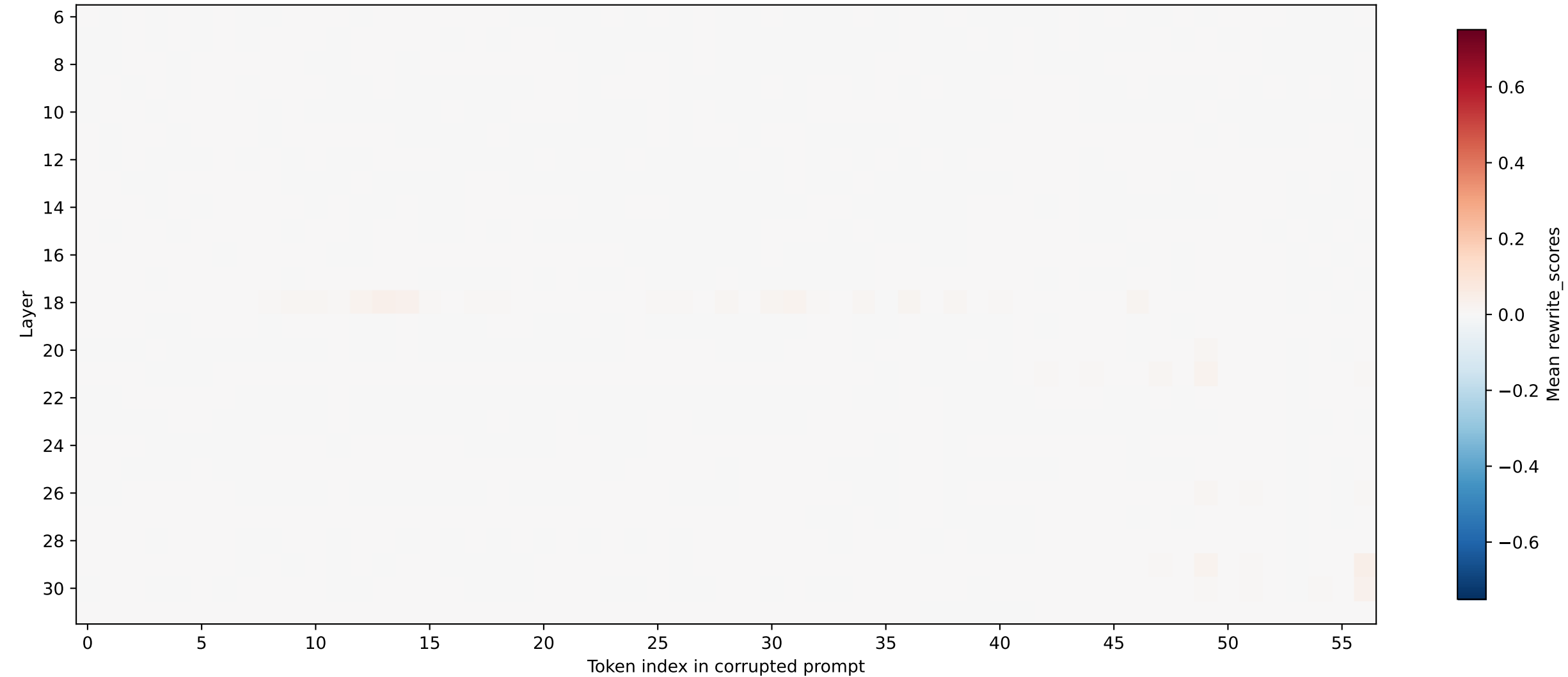
OLMo all conditions/prompts: mean rewrite_scores by layer and token index (layers 6 plus)
