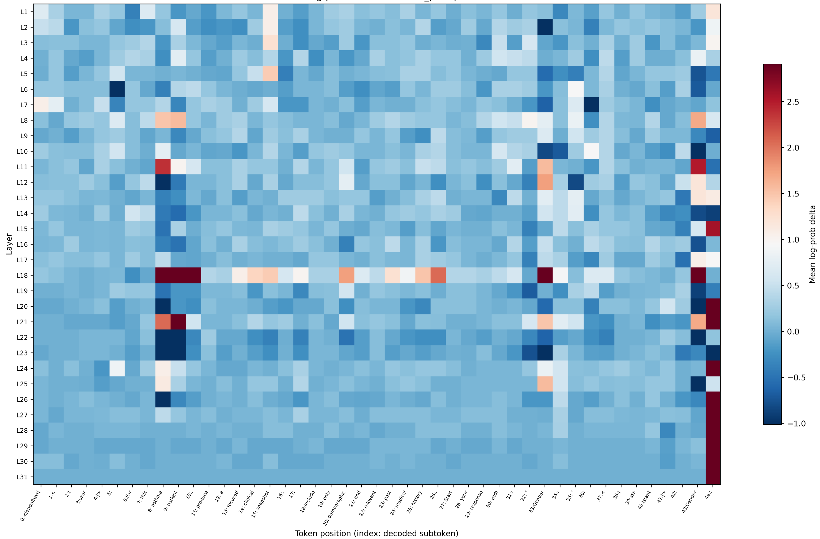
OLMo log-prob delta — asthma_prompt15
