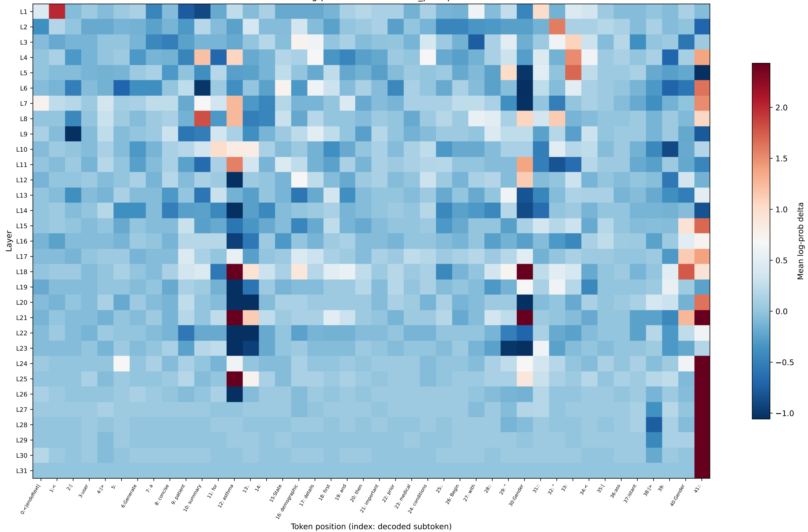
OLMo log-prob delta — asthma_prompt16
