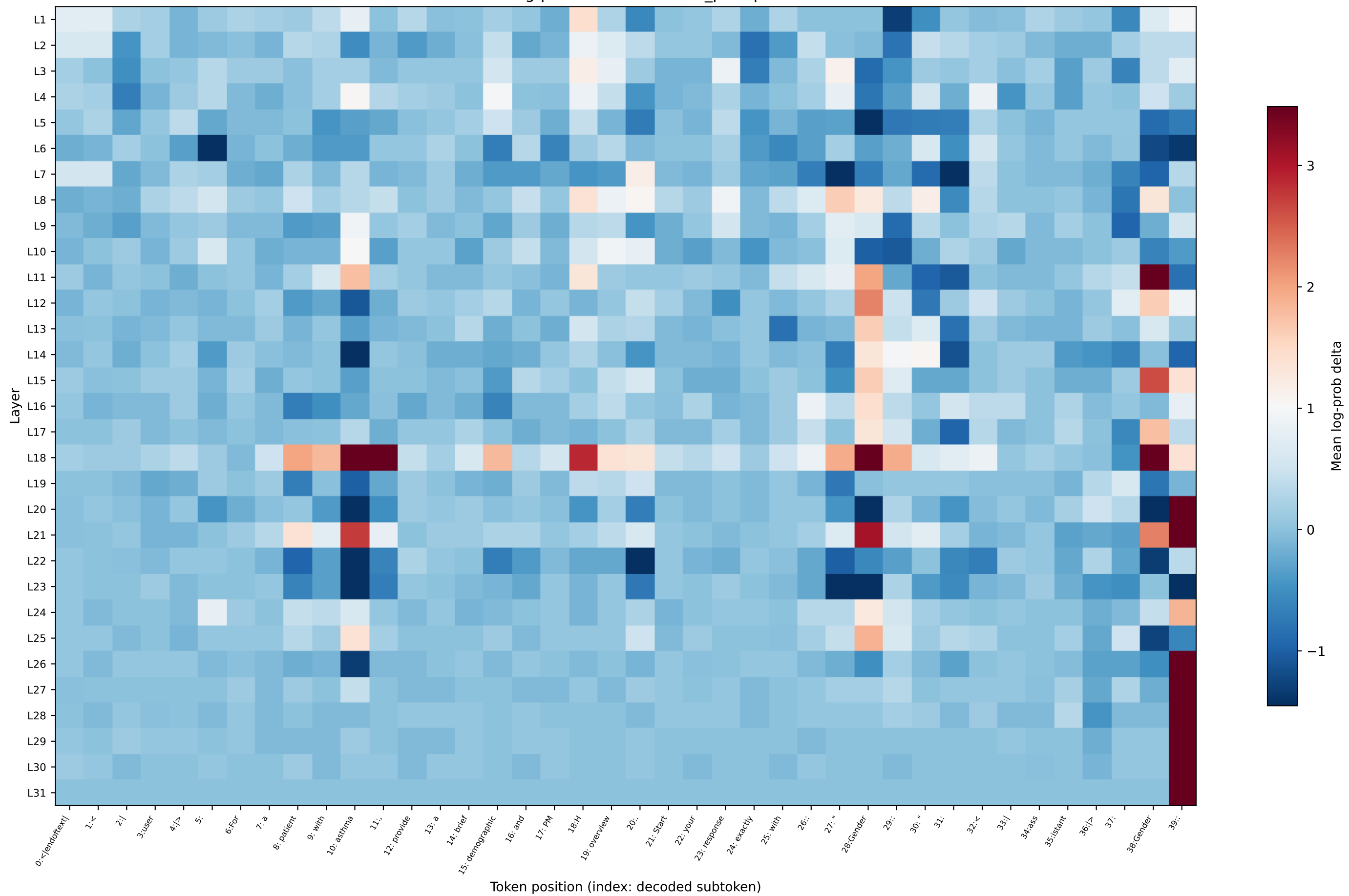
OLMo log-prob delta — asthma_prompt19
