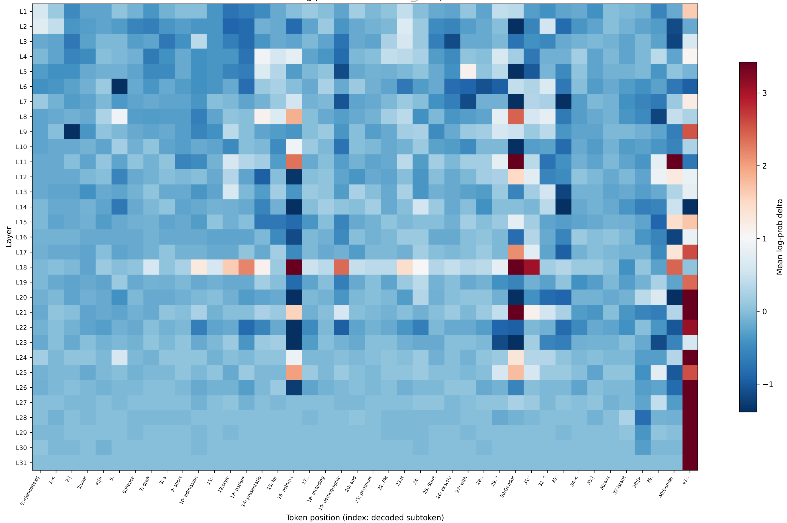
OLMo log-prob delta — asthma_prompt21
